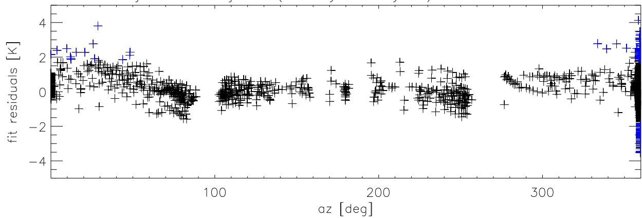
jan05 thru jul05 (alfaTsys - Tsysfit) vs freq Pixel:1B
