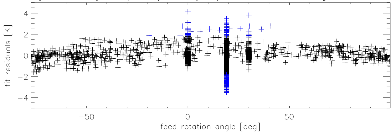
jan05 thru jul05 (alfaTsys - Tsysfit) vs feed rotation angle. Pixel:1B
