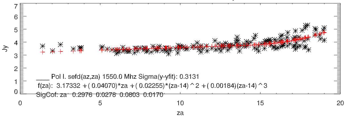
lbw 1550 sefd vs za and fit dec17-jun18
