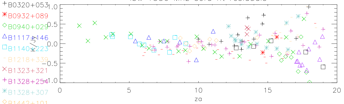
lbw 1610 Mhz sefd fit residuals
