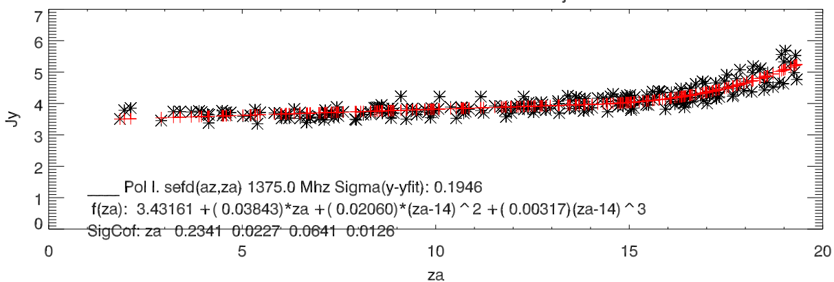
lbw 1375 sefd vs za and fit dec17-jun18
