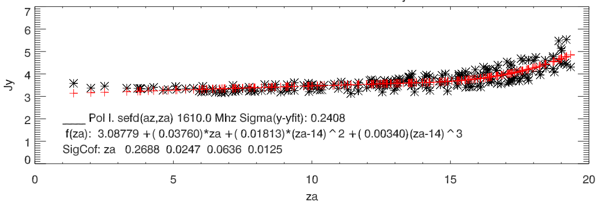
lbw 1610 sefd vs za and fit dec17-jun18
