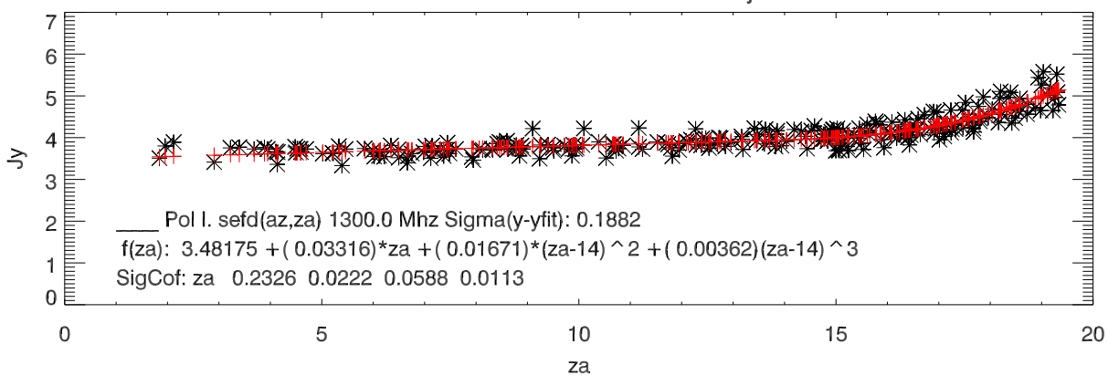
lbw 1300 sefd vs za and fit dec17-jun18
