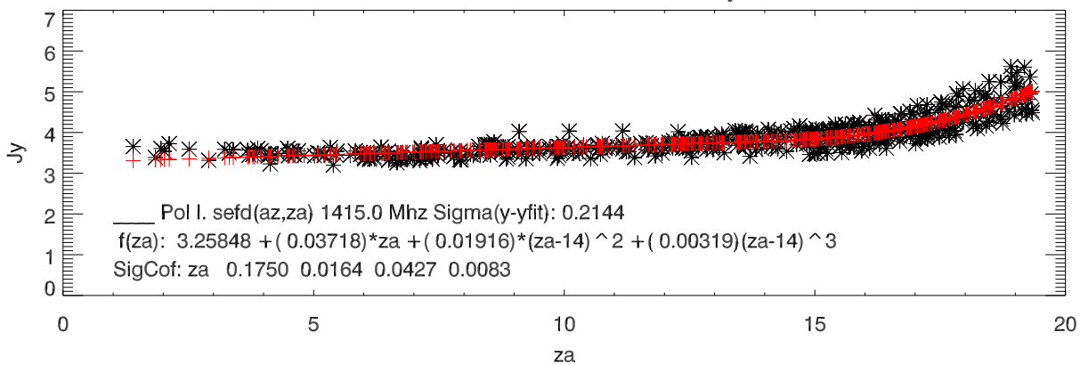
lbw 1415 sefd vs za and fit dec17-jun18
