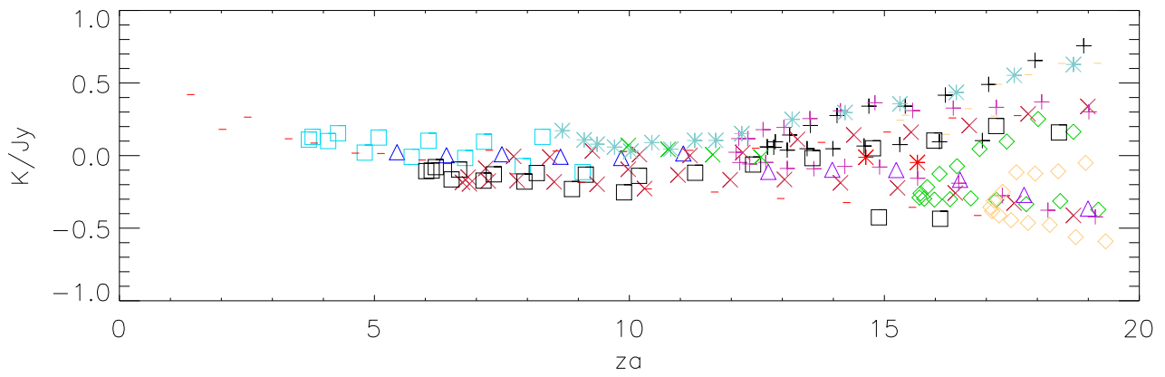
lbw 1666 Mhz sefd fit residuals
