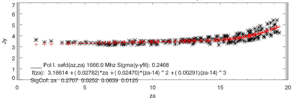
lbw 1666 sefd vs za and fit dec17-jun18
