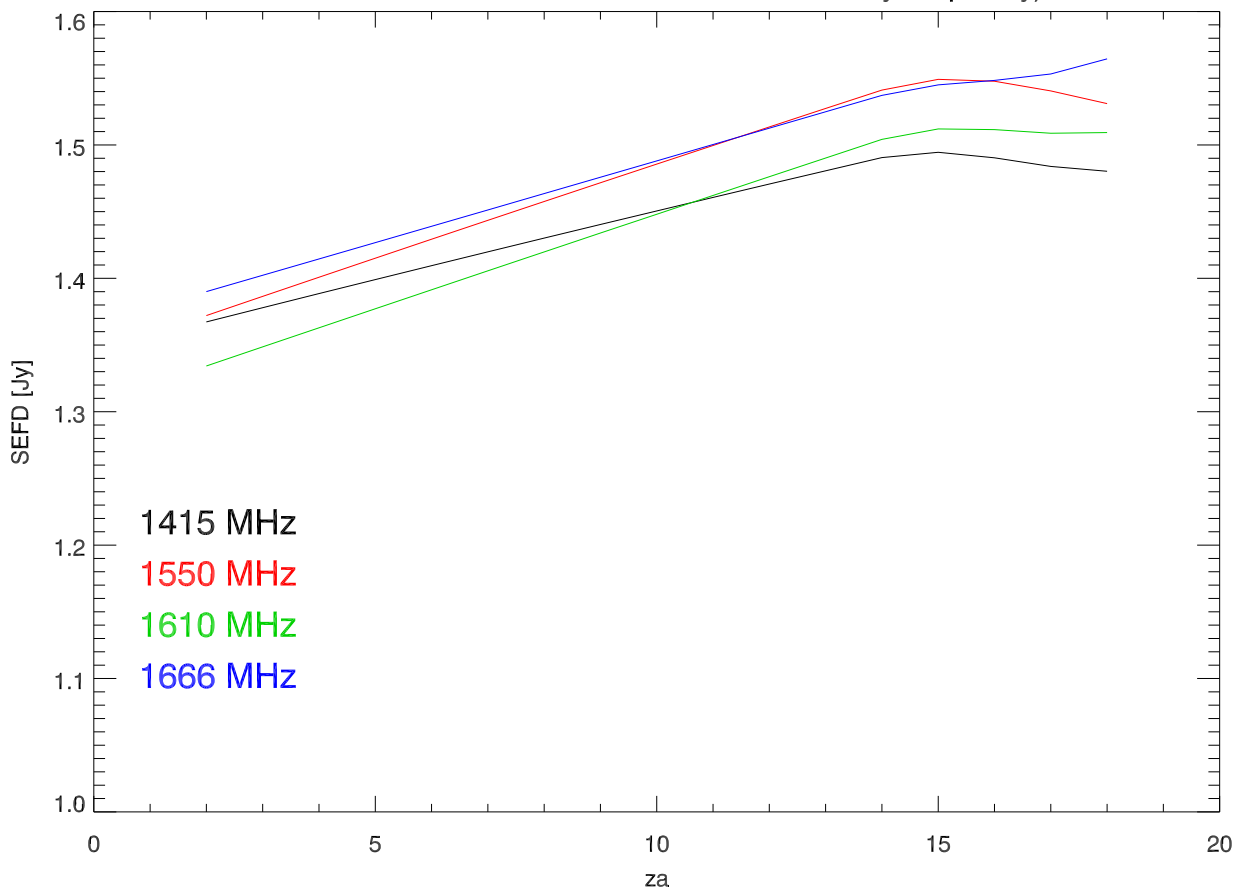
Ratio of PostMariaSEFD/PreMariaSEFD vs za by frequency)
