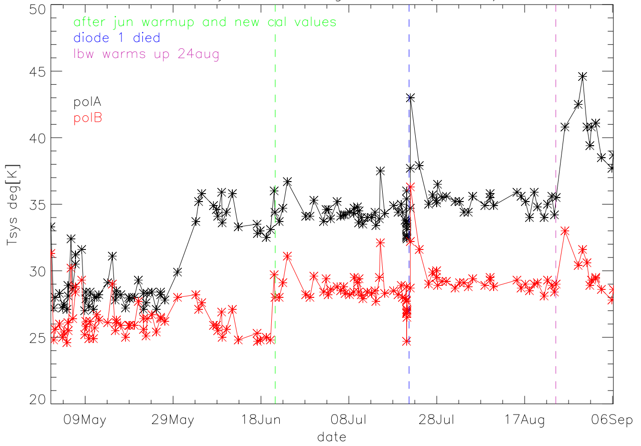
lbw Tsys 2005 using diode 2 (h90cal)
