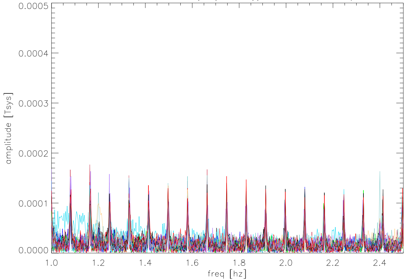
A2013 lbwPoIB abs(fft(totPwr)). 53 5 min strips
