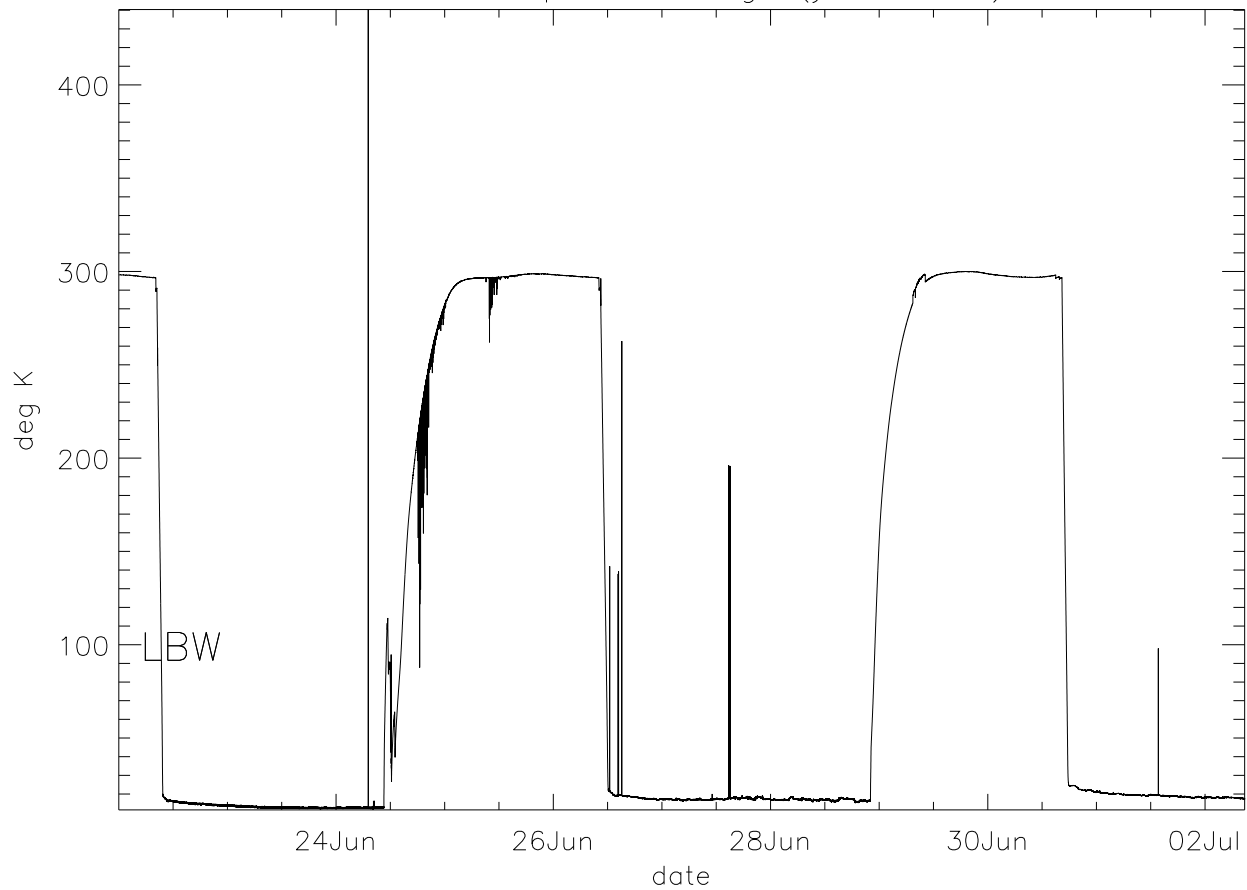
Dewar temps 16K stage (year 2008)
