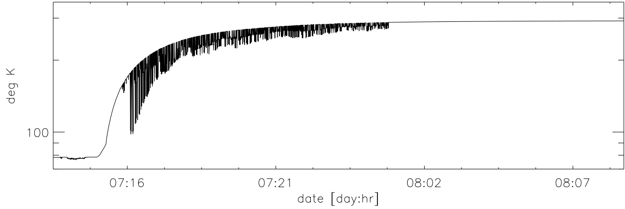
omt blowup at end of warmup: linear scale
