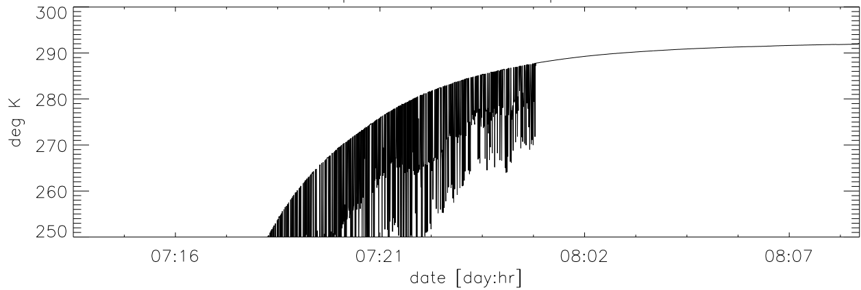
16K stage temp vs time : log scale
