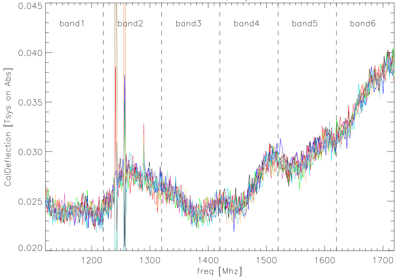
23nov05 lbw calDeflection/Tsys on Absorber polB
