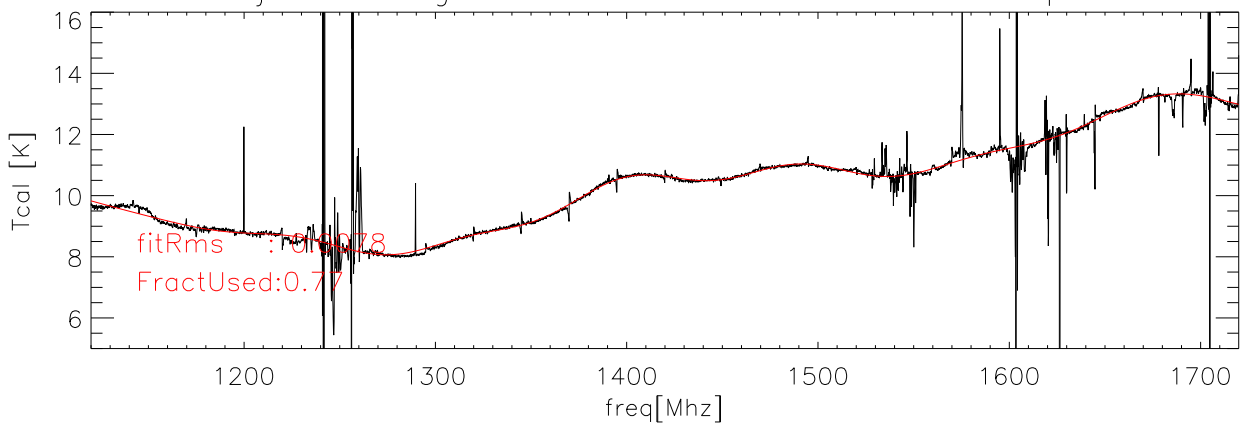
06jul06 Averaged data and fit for Tcal Kelvins hxcal polA
