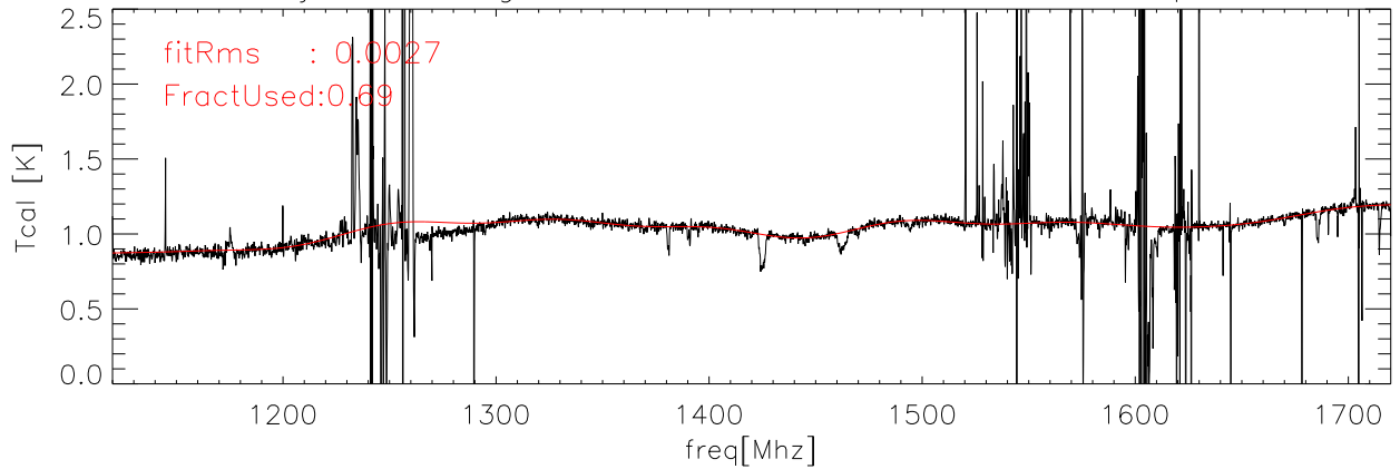
06jul06 Averaged data and fit for Tcal Kelvins lcor polB
