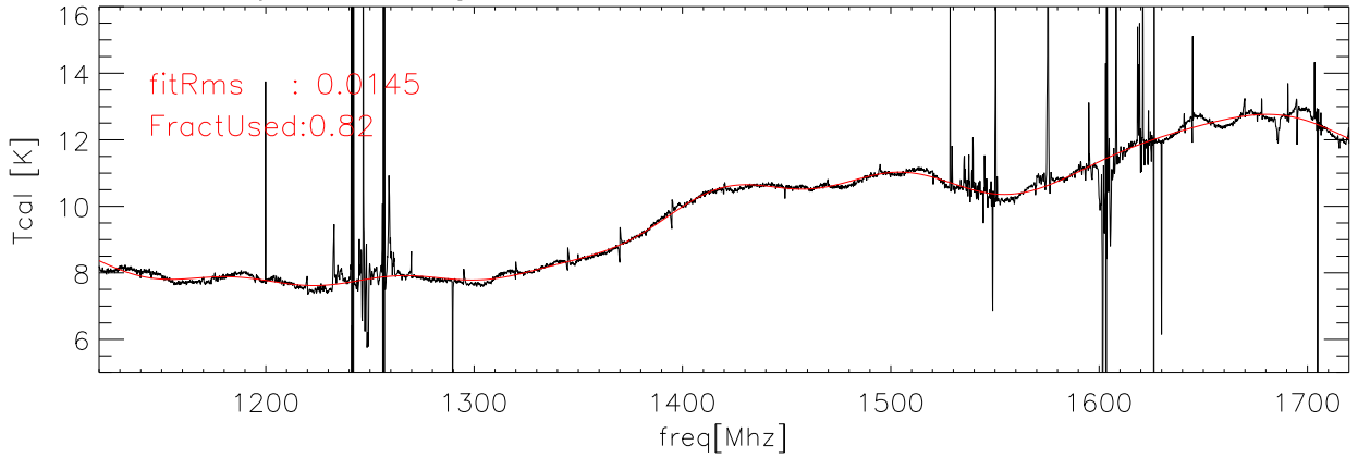
06jul06 Averaged data and fit for Tcal Kelvins h90cal polB
