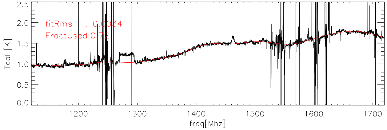
06jul06 Averaged data and fit for Tcal Kelvins I90cal polB
