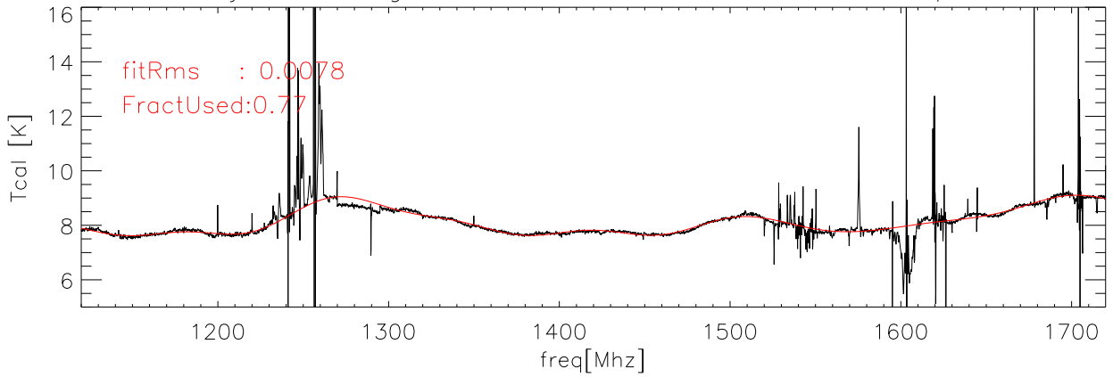
06jul06 Averaged data and fit for Tcal Kelvins hcal polB
