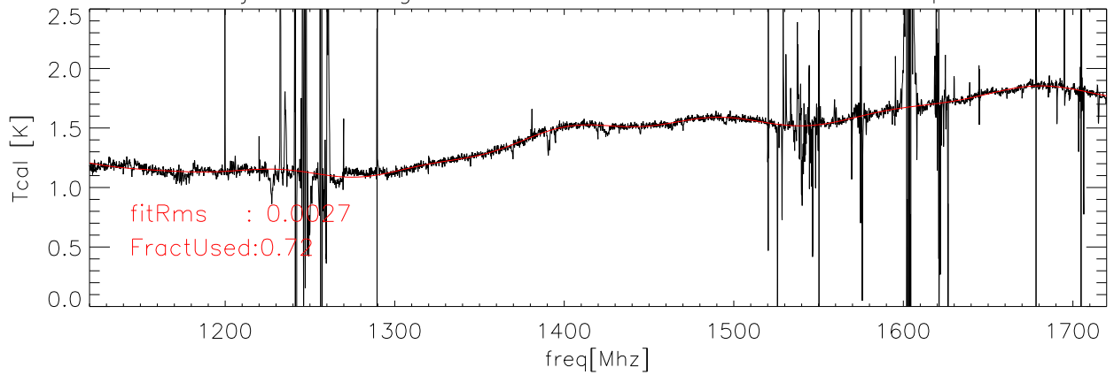
06jul06 Averaged data and fit for Tcal Kelvins lxcal polA
