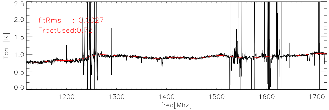
06jul06 Averaged data and fit for Tcal Kelvins lcal polB
