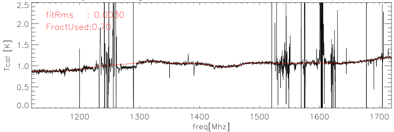
06jul06 Averaged data and fit for Tcal Kelvins lxcal polB
