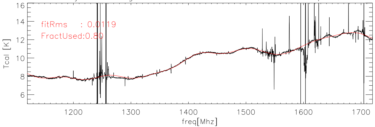
06jul06 Averaged data and fit for Tcal Kelvins hxcal polB
