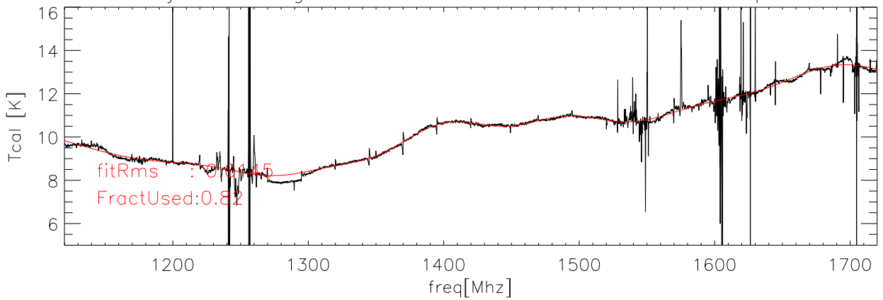
06jul06 Averaged data and fit for Tcal Kelvins lcor polA
