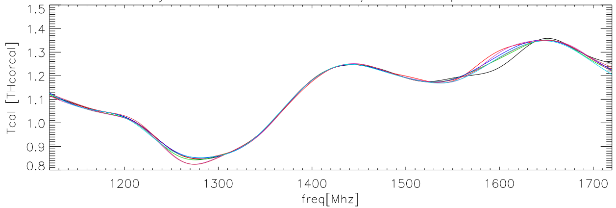
06jul06 OverPlot fits to TCal/Thcorcal polA hxcal
