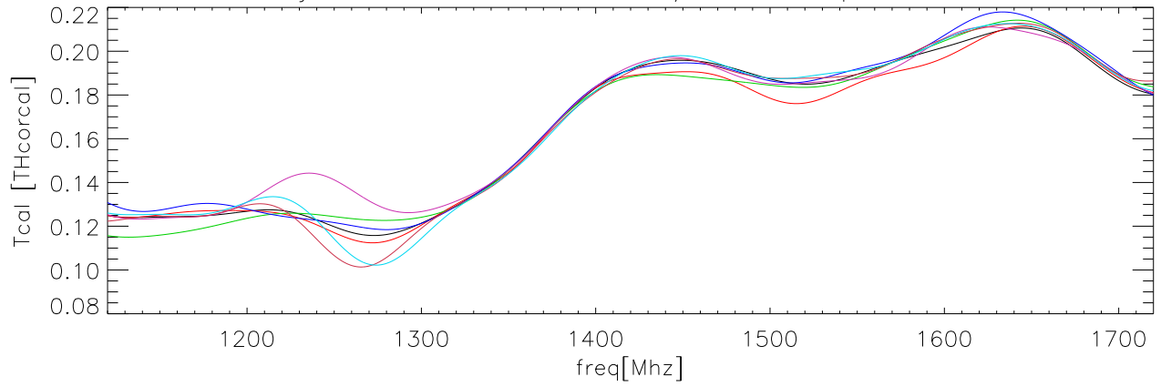
06jul06 OverPlot fits to TCal/Thcorcal polB I90cal
