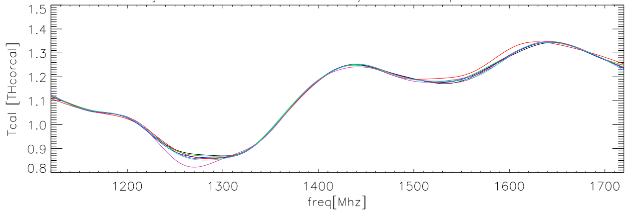
06jul06 OverPlot fits to TCal/Thcorcal polA lcor
