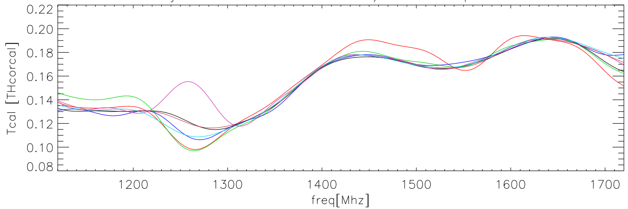
06jul06 OverPlot fits to TCal/Thcorcal polA lxccl
