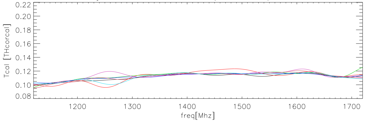
06jul06 OverPlot fits to TCal/Thcorcal polB lxccl
