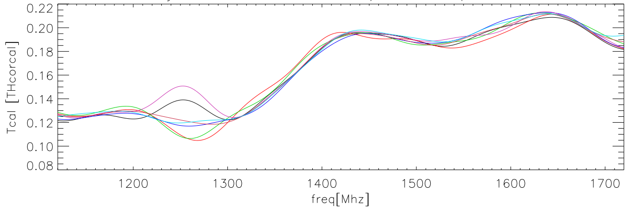
06jul06 OverPlot fits to TCal/Thcorcal polB lxccl
