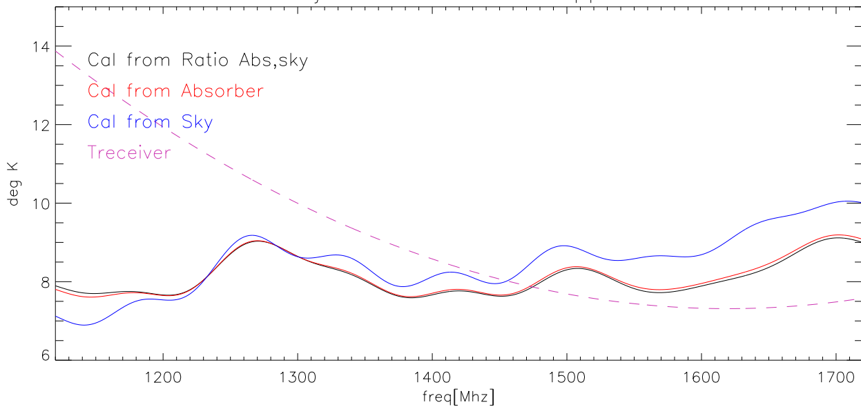
06jul06 Cal in Kelvins vs freq polB
