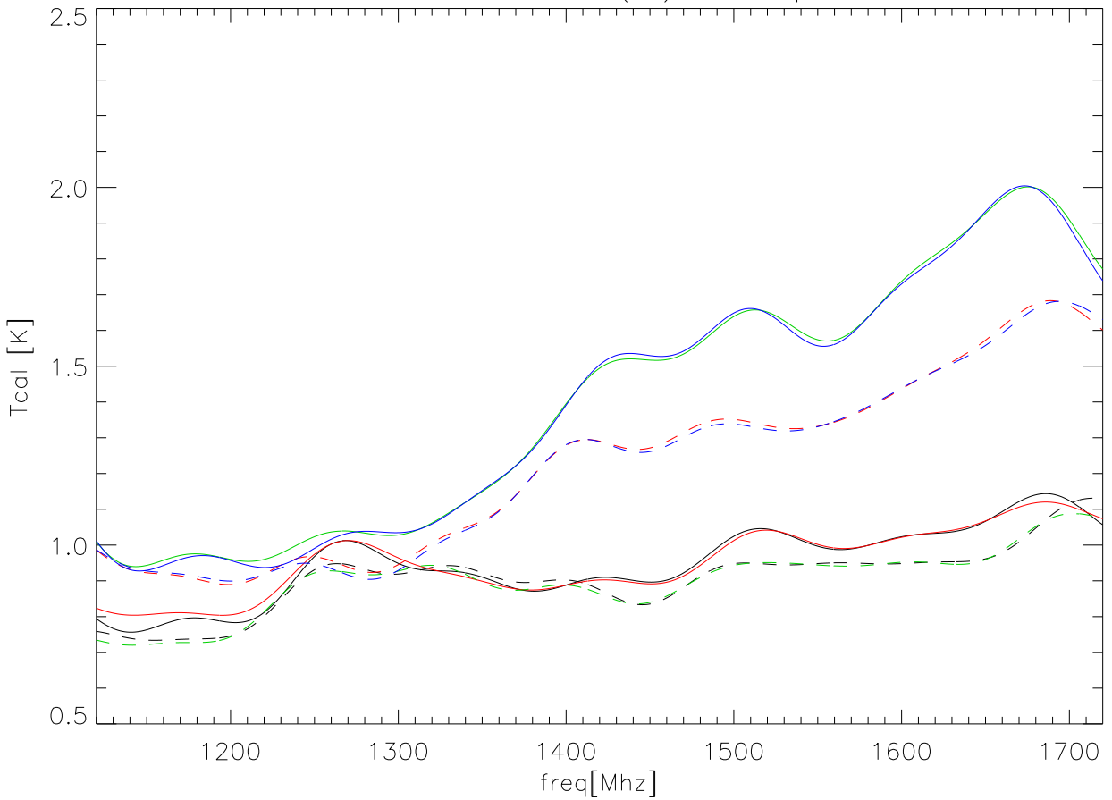
23feb06 Cal In Kelvins (fit) vs freq Low cal
