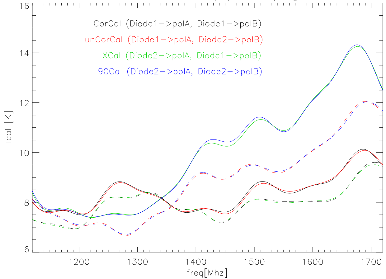
23feb06 Cal In Kelvins (fit) vs freq Low cal
