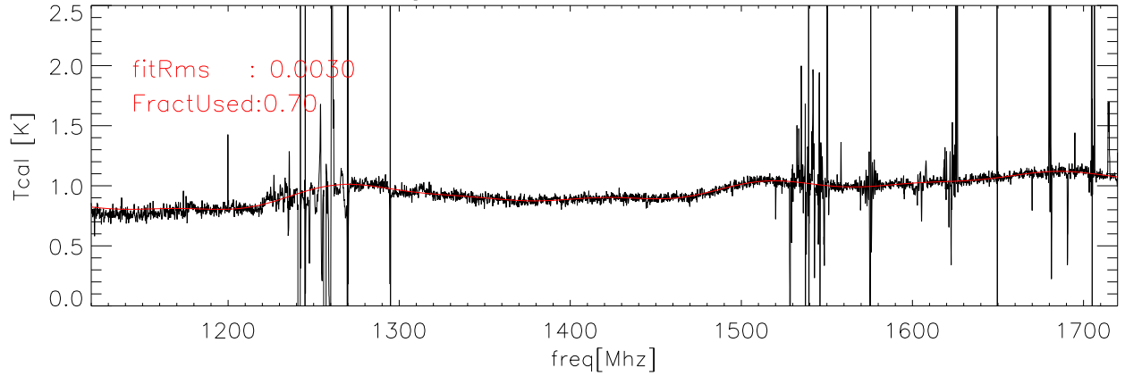
23feb06 Averaged data and fit for Tcal Kelvins lcal polB
