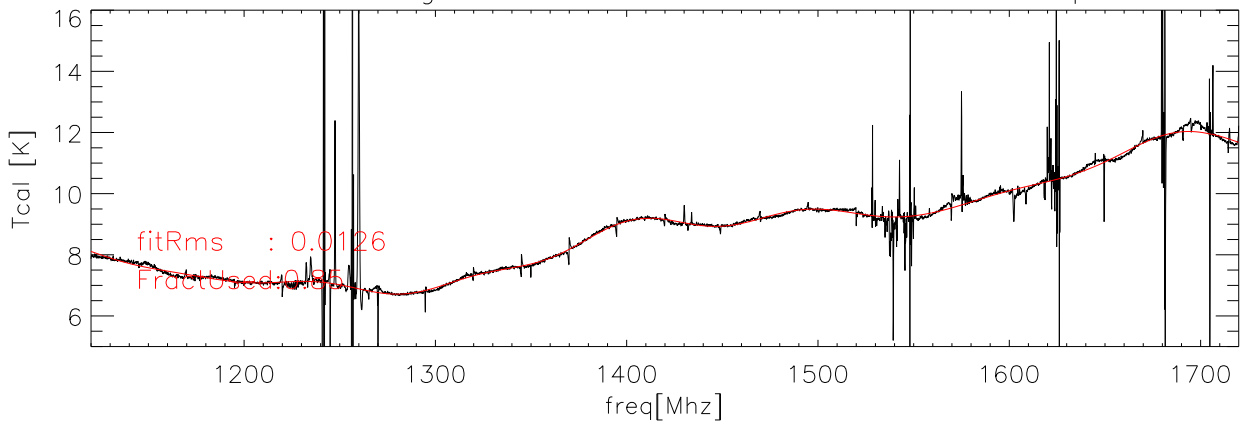
23feb06 Averaged data and fit for Tcal Kelvins lcor poA
