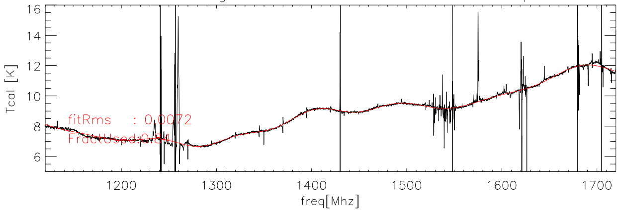
23feb06 Averaged data and fit for Tcal Kelvins hxcal polA
