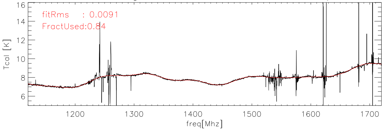
23feb06 Averaged data and fit for Tcal Kelvins hxcal polB
