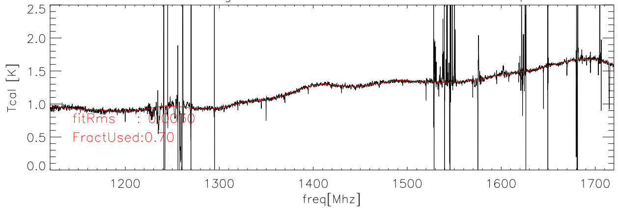
23feb06 Averaged data and fit for Tcal Kelvins lxcal polA
