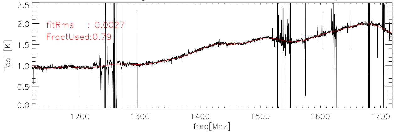
23feb06 Averaged data and fit for Tcal Kelvins lxcal polB
