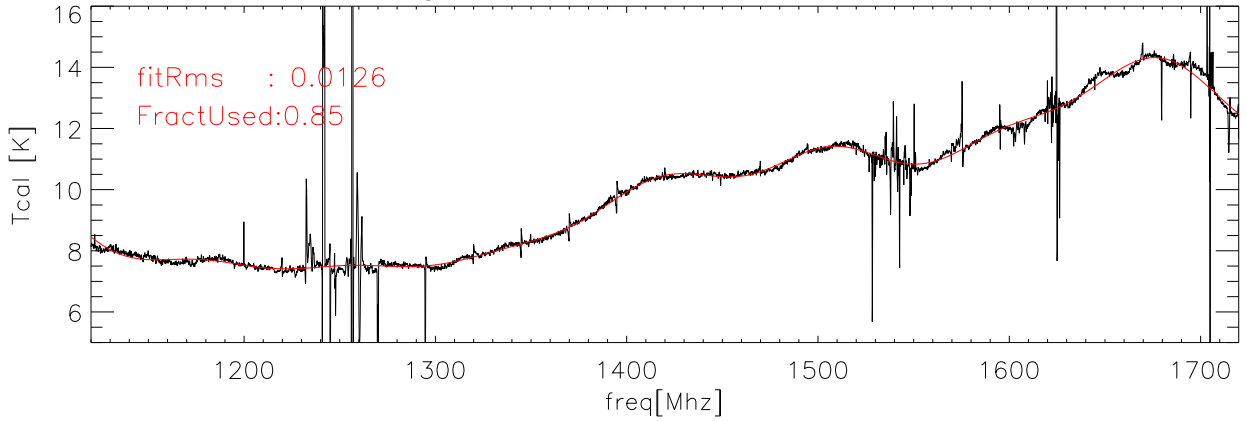
23feb06 Averaged data and fit for Tcal Kelvins h90cal poB
