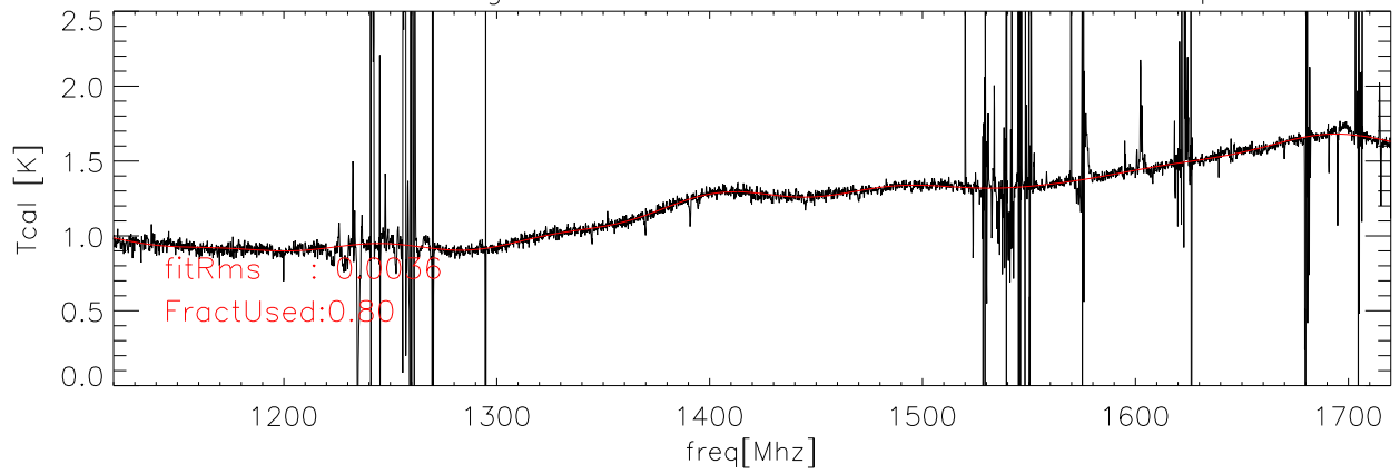
23feb06 Averaged data and fit for Tcal Kelvins I90cal polB
