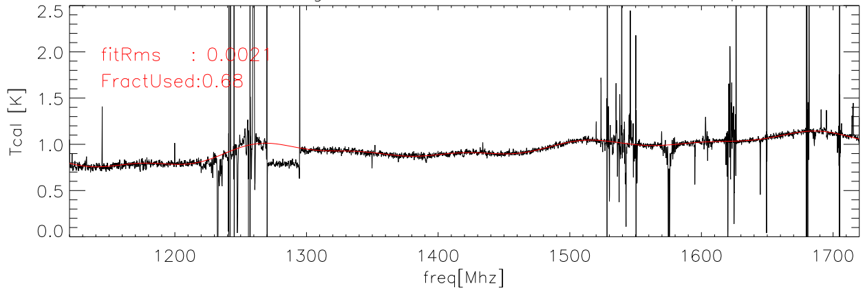
23feb06 Averaged data and fit for Tcal Kelvins lcor poB
