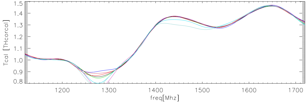
23feb06 OverPlot fits to TCal/Thcorcal polB h90cal
