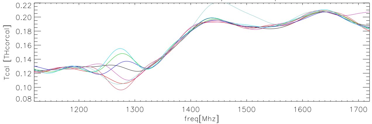
23feb06 OverPlot fits to TCal/Thcorcal polB lxccl
