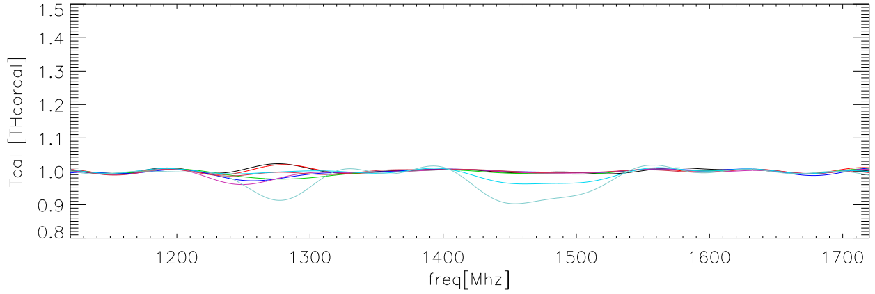
23feb06 OverPlot fits to TCal/Thcorcal polB hcal
