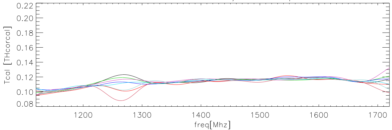
23feb06 OverPlot fits to TCal/Thcorcal polB lxccl
