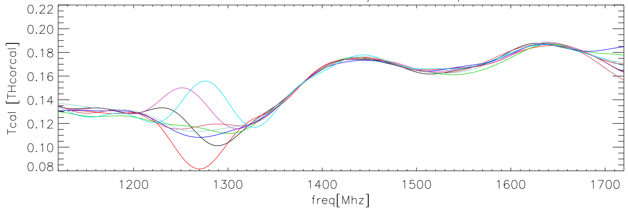
23feb06 OverPlot fits to TCal/Thcorcal polB I90cal
