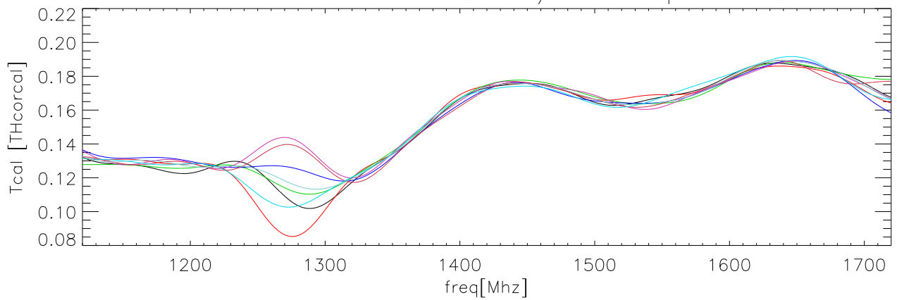
23feb06 OverPlot fits to TCal/Thcorcal polA lxccl
