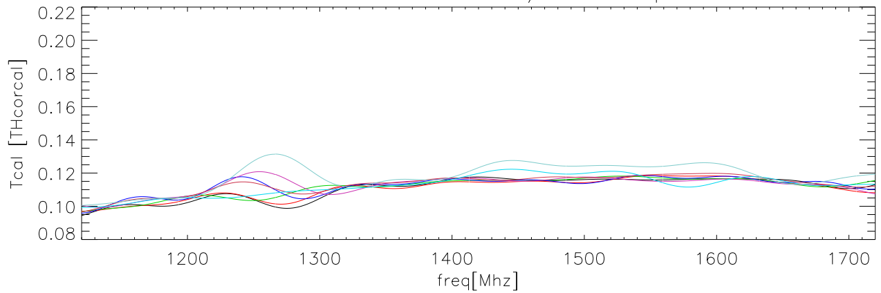
23feb06 OverPlot fits to TCal/Thcorcal polB lcor
