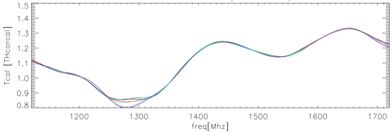
23feb06 OverPlot fits to TCal/Thcorcal polA hxccl
