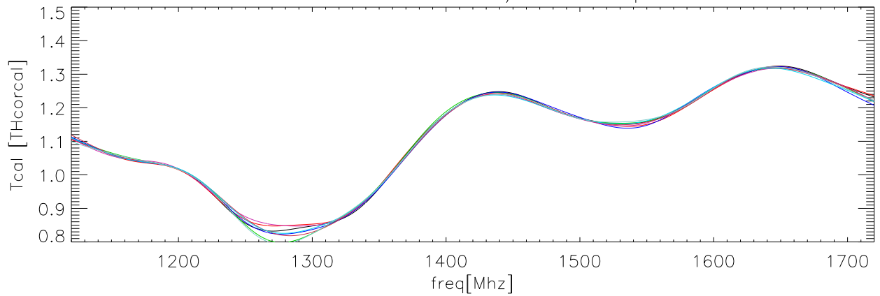
23feb06 OverPlot fits to TCal/Thcorcal polA lcor
