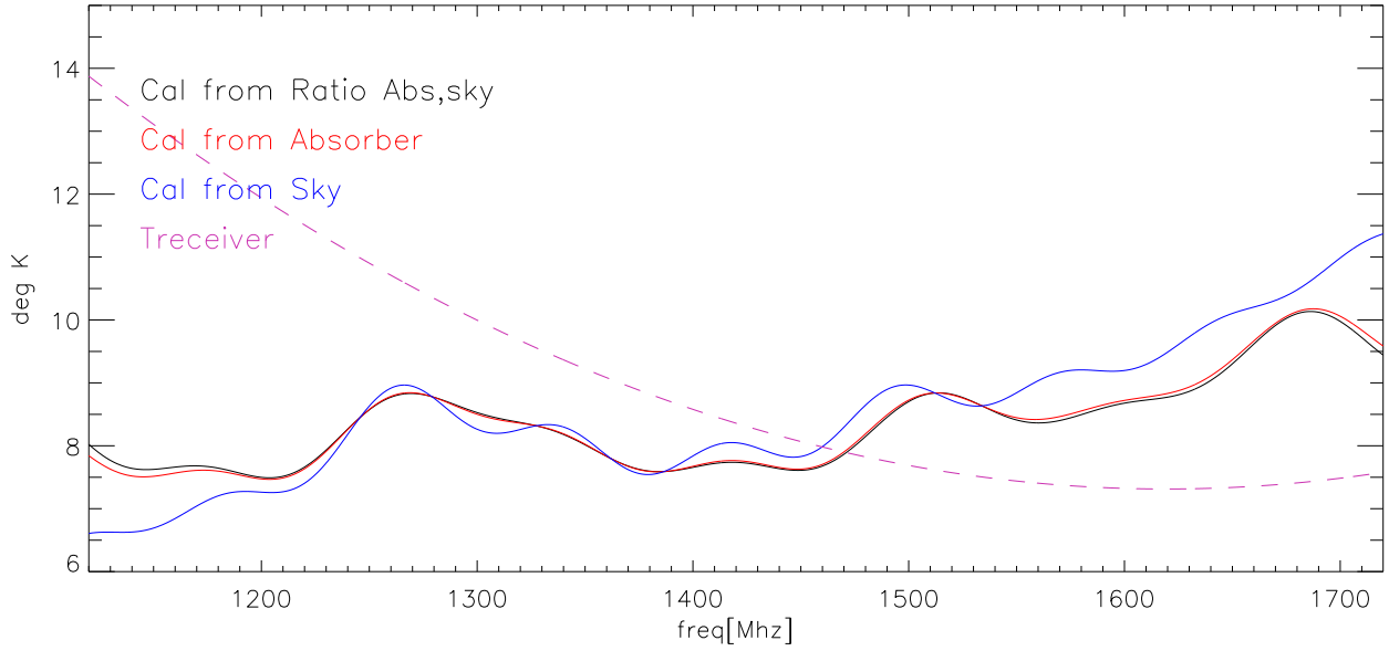
23feb06 Cal in Kelvins vs freq polB
