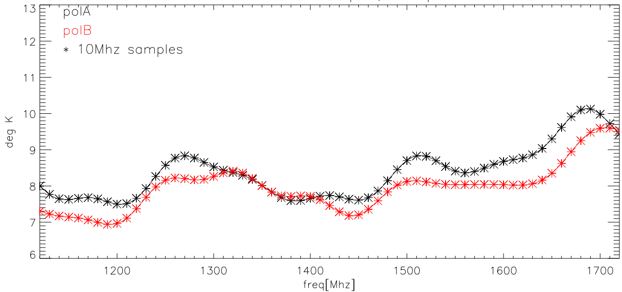
23feb06 Cal in Kelvins polA,B overplotted
