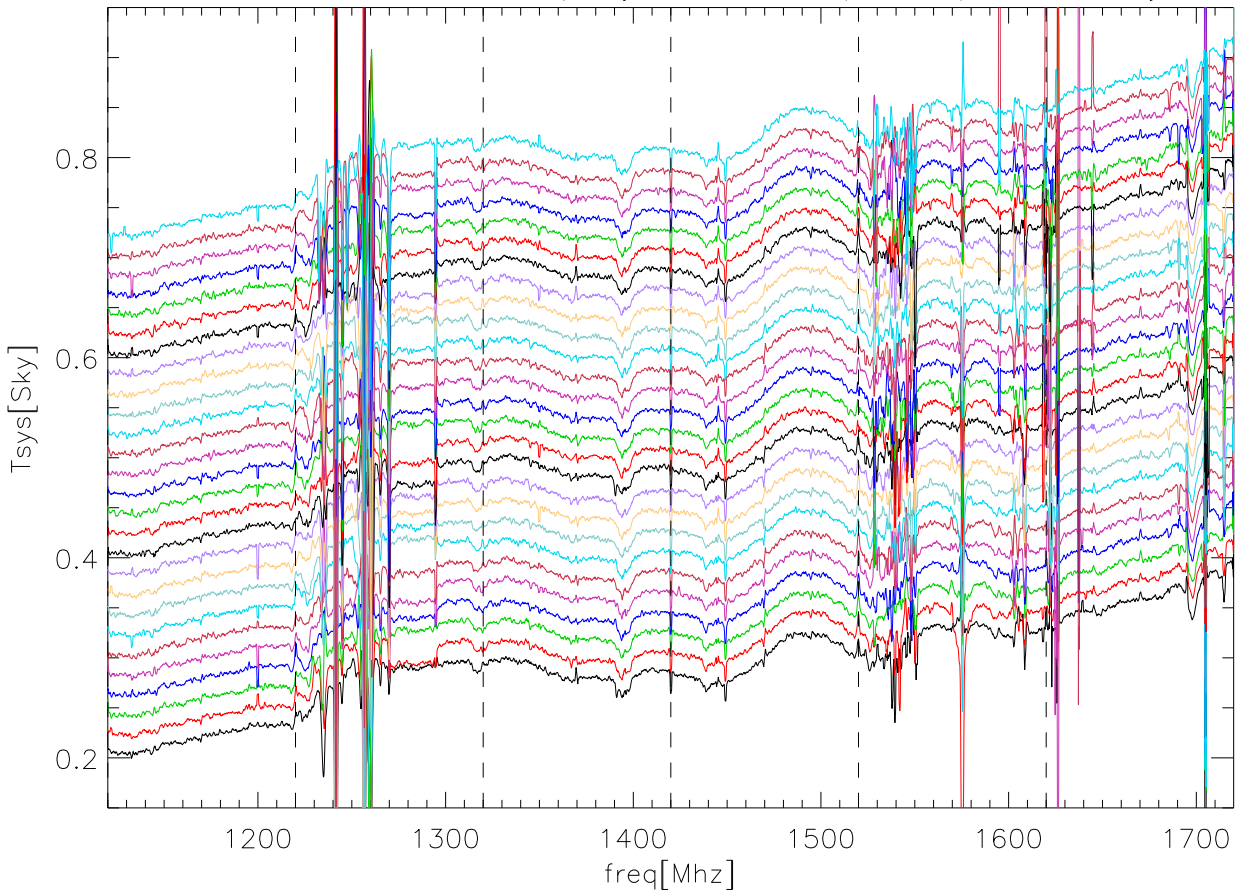
23feb06 CalDeFlection/Tsys for each pass polB on Sky
