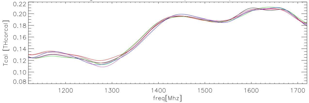
29aug08 OverPlot fits to TCal/Thcorcal polB lxccl
