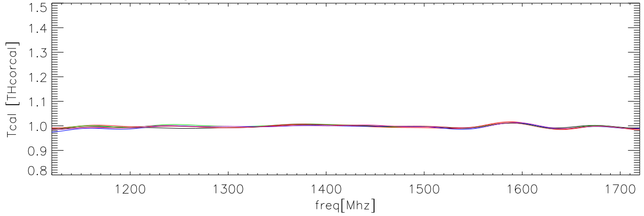
29aug08 OverPlot fits to TCal/Thcorcal polB hcal
