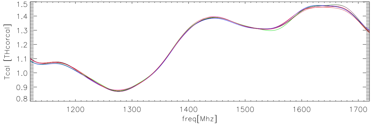
29aug08 OverPlot fits to TCal/Thcorcal polB h90cal
