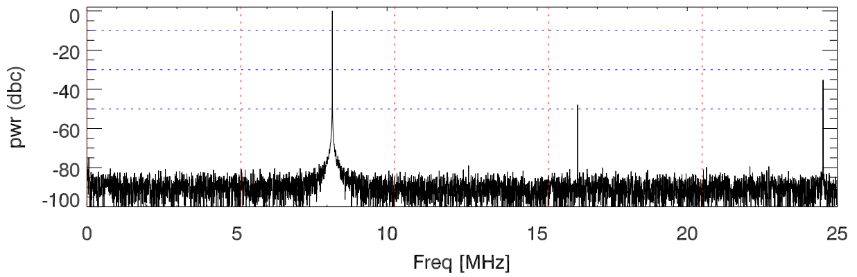
170223 tx3 tube monitor ports: spectral density. BroadBand
