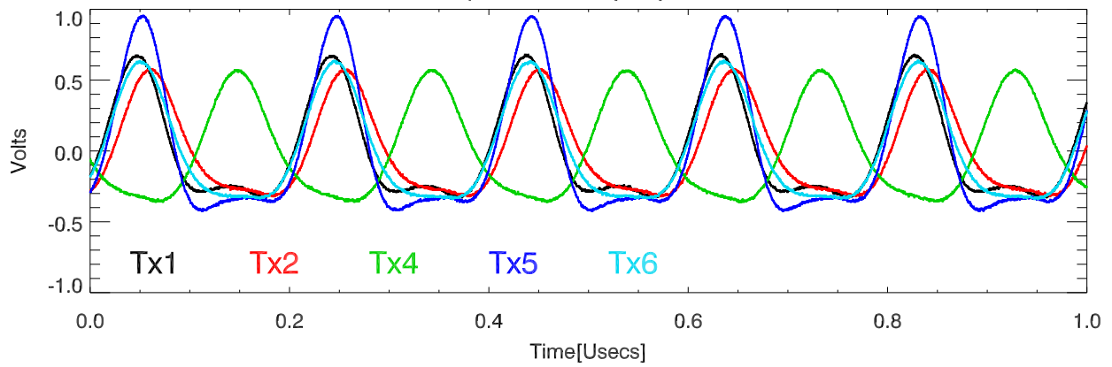
170207 overplot tube output ports. IPA Anode
