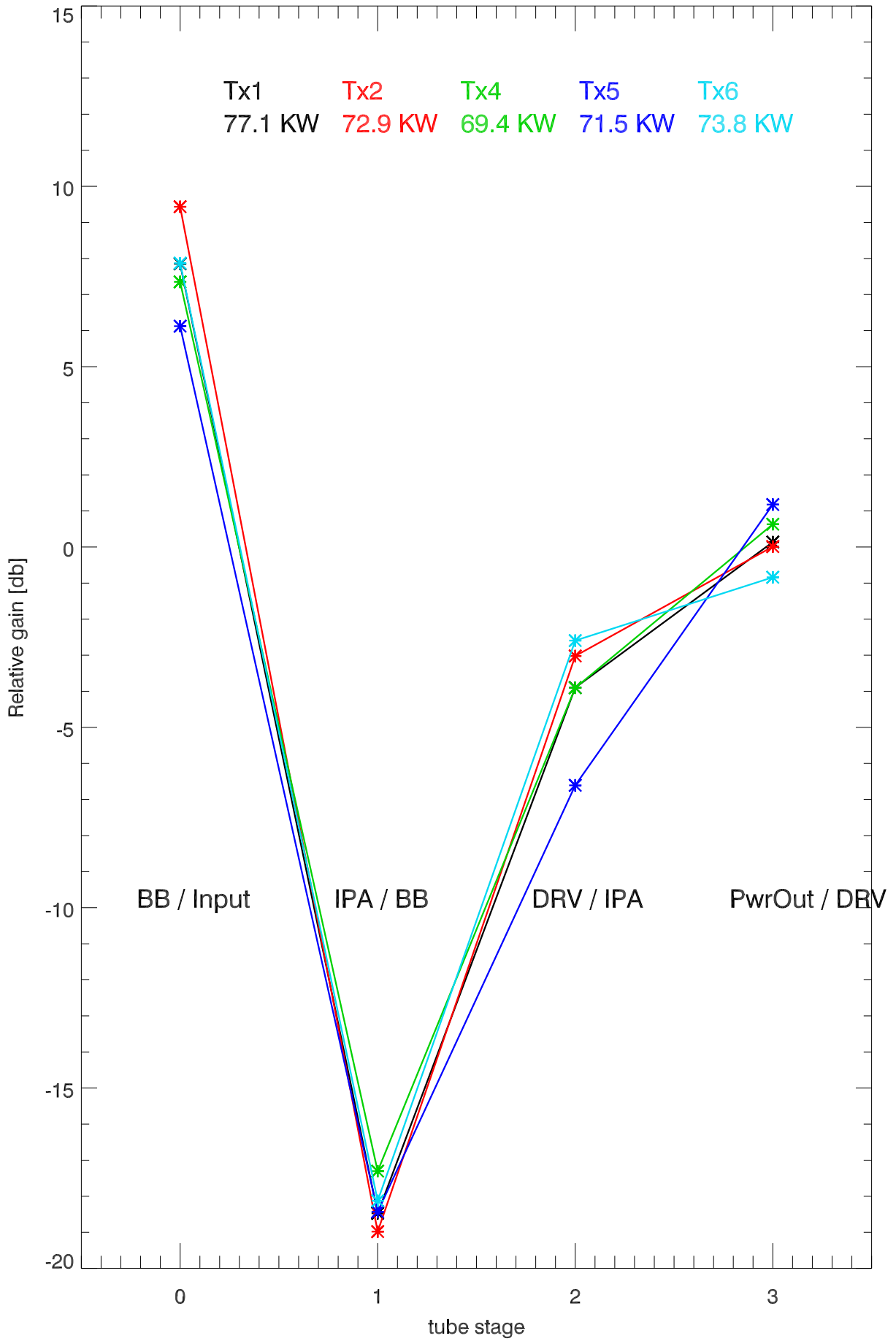
170207 relative gain of tube stages. (PwrOut[n+1]/PwrOut[n])
