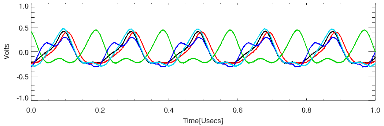
170207 overplot tube output ports. Driver Anode
