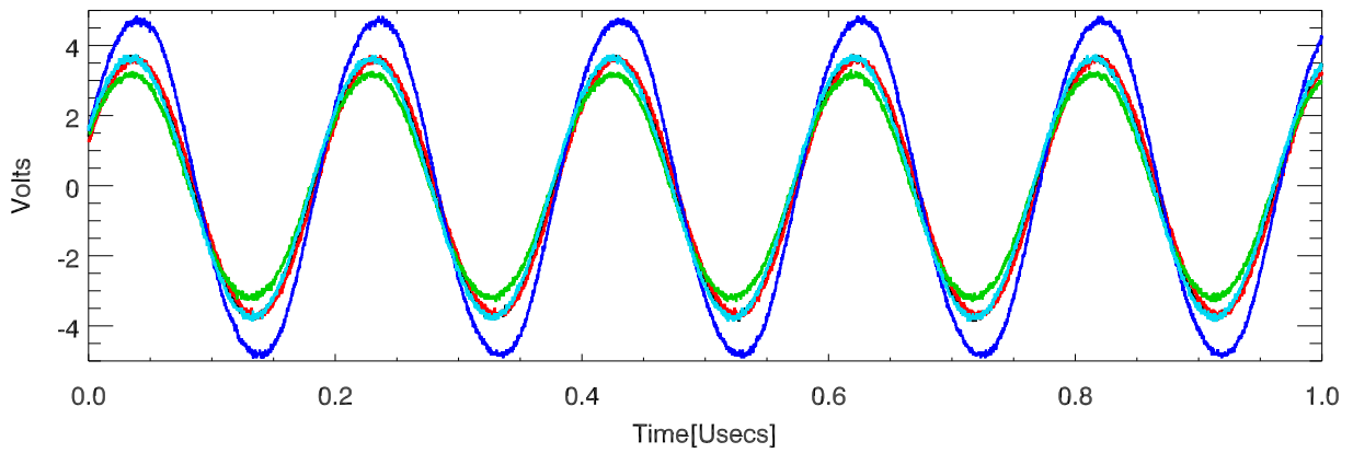
170207 overplot tube output ports. IPA Anode
