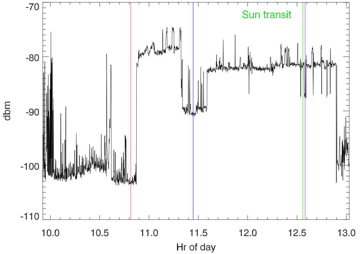
31jul18 average totPwr (100KHz about 8.175Mhz) vs hr of day
