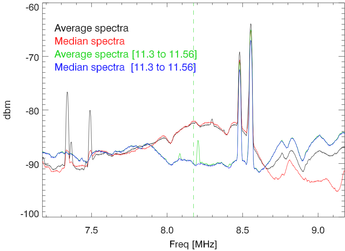
31jul18 average spectra. hf 8Mhz dipole 1. RBW=10KHz
