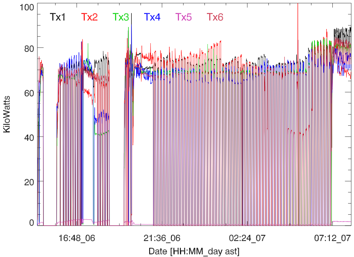
TxPwr by Tx. 06nov16:T2873. Juha Vierinen
