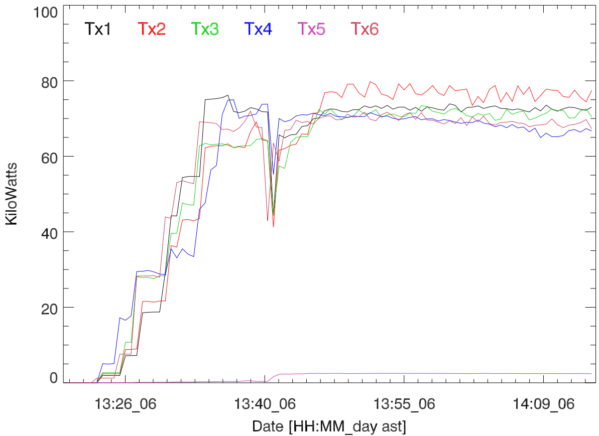
TxPwr by Tx. 06oct16:T2566. Paul BernHardt
