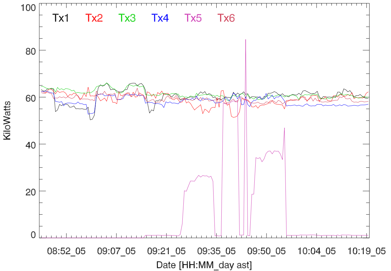
TxPwr by Tx. 05oct16:T2915. Salih Bostan
