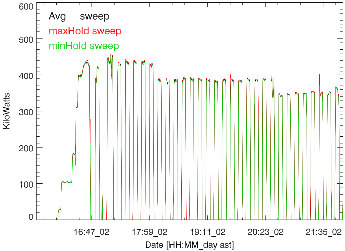
TxPwrTot. 02oct16:H3112. Elizabeth Kendall 5 MHz
