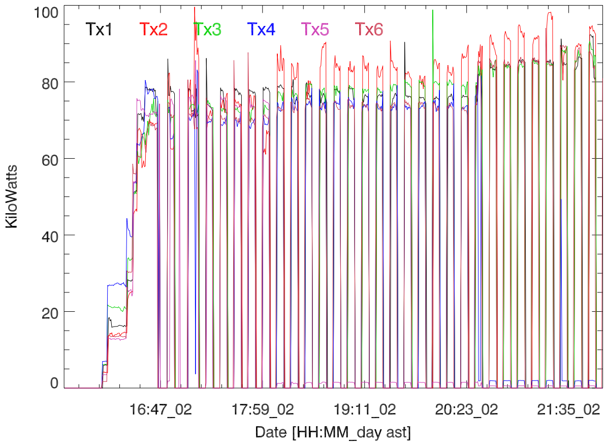
TxPwr by Tx. 02oct16:H3112. Elizabeth Kendall
