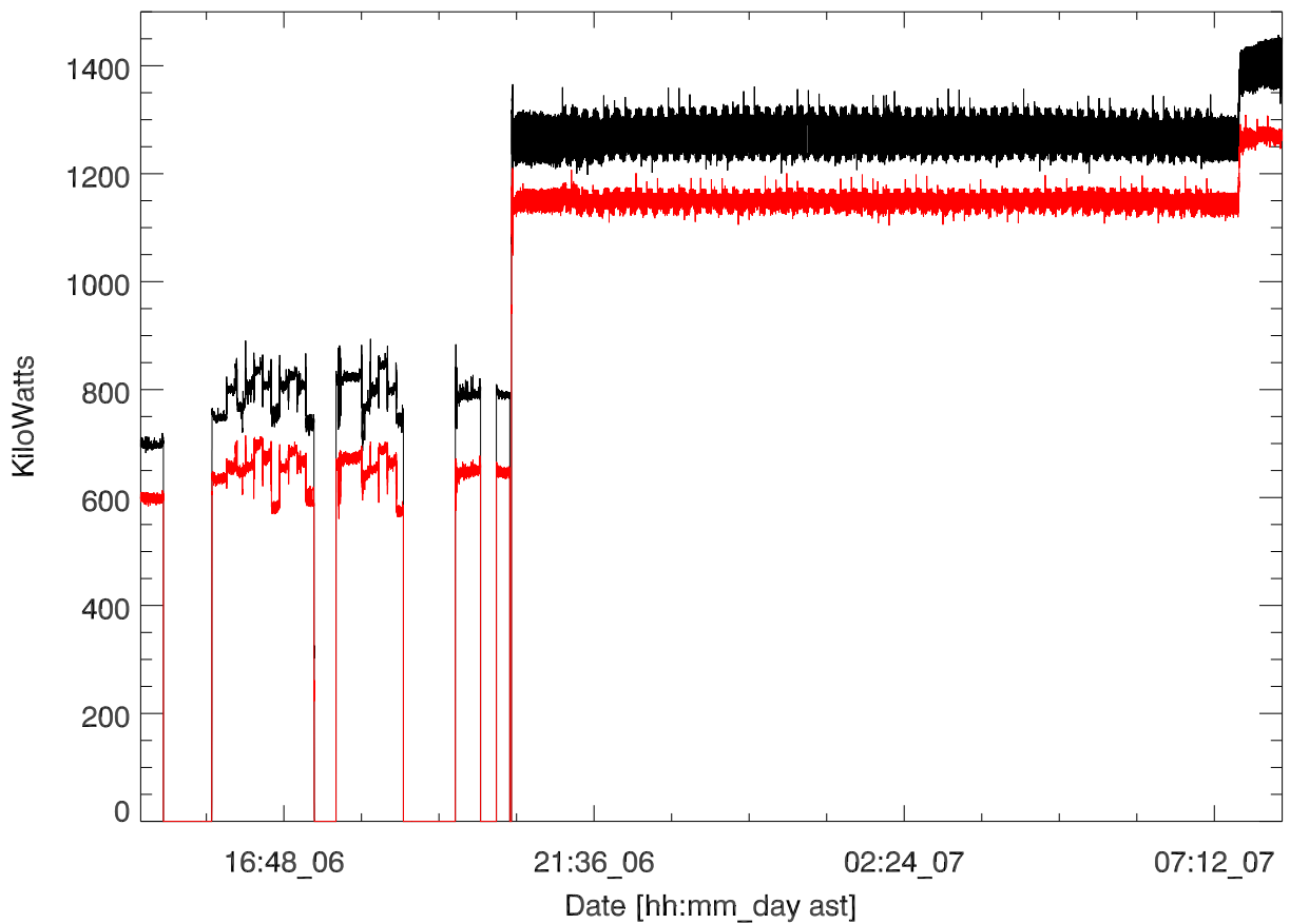
GD 430 Transmitted power for: 06nov16:T2873. Juha Vierinen
