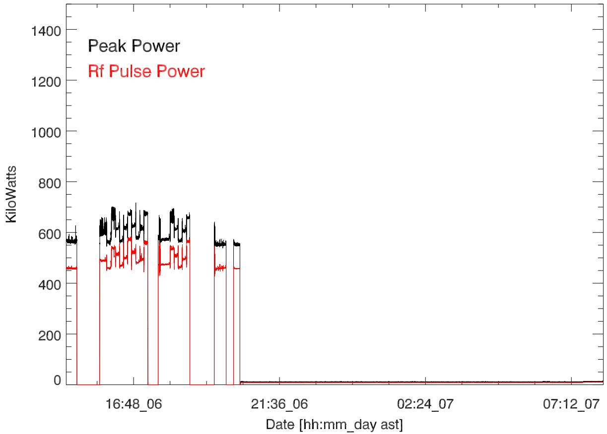
CH 430 Transmitted power for: 06nov16:T2873. Juha Vierinen
