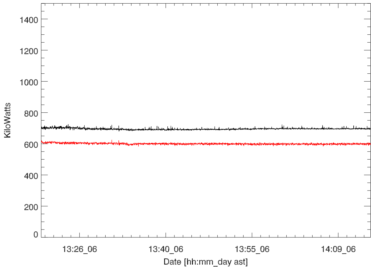
GD 430 Transmitted power for: 06oct16:T2566. Paul Bernhardt
