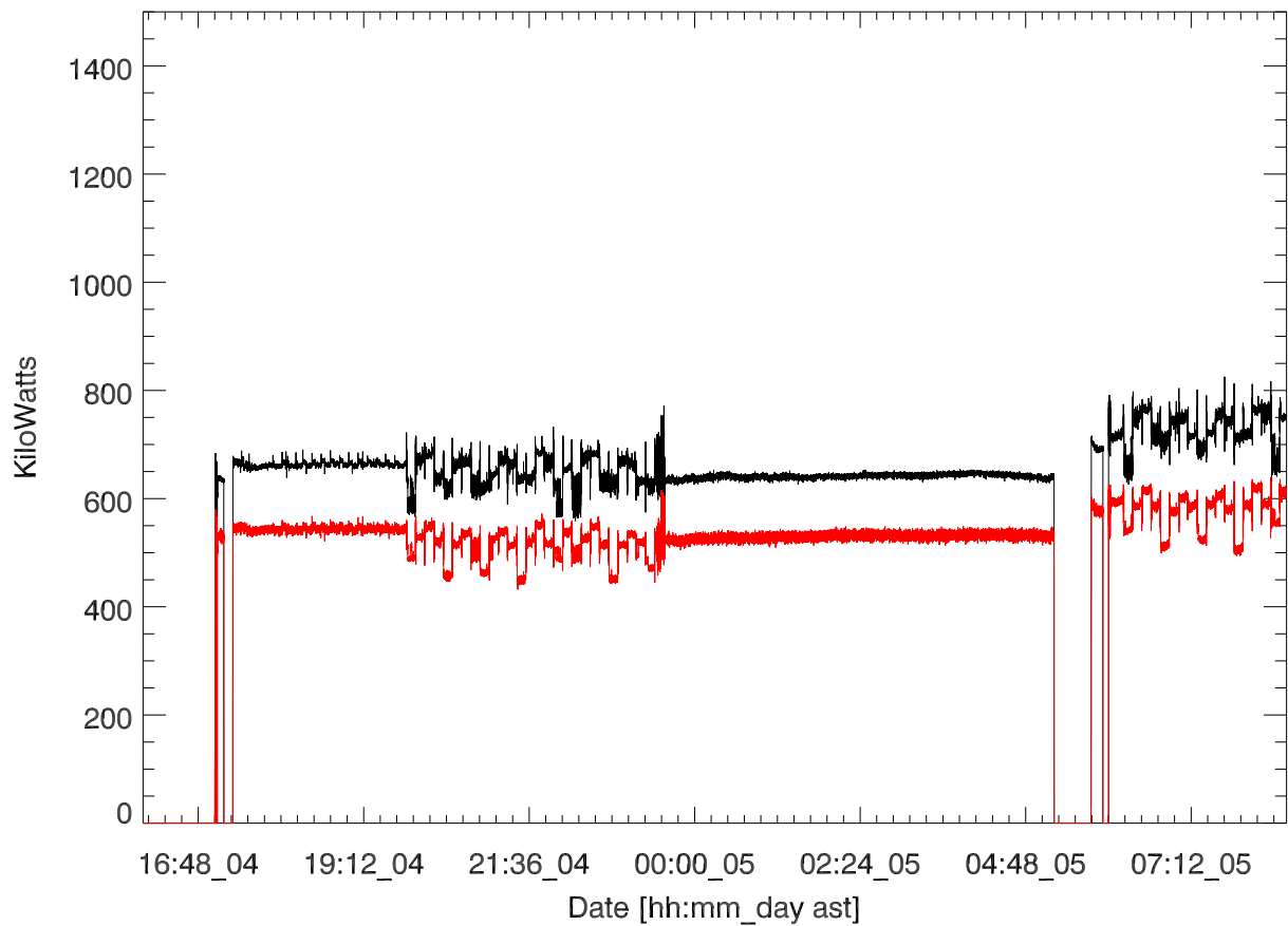
GD 430 Transmitted power for: 04nov16:T2873. Juha Vierinen
