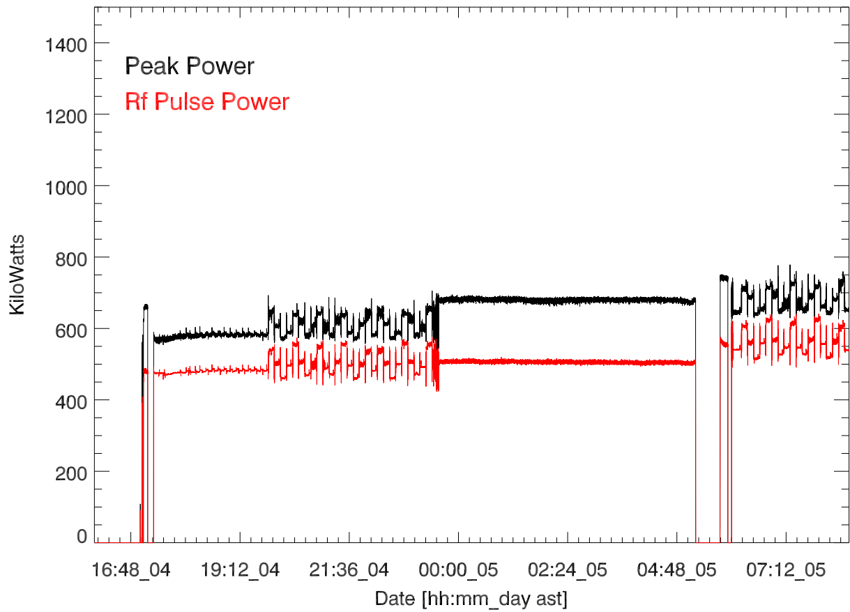
CH 430 Transmitted power for: 04nov16:T2873. Juha Vierinen
