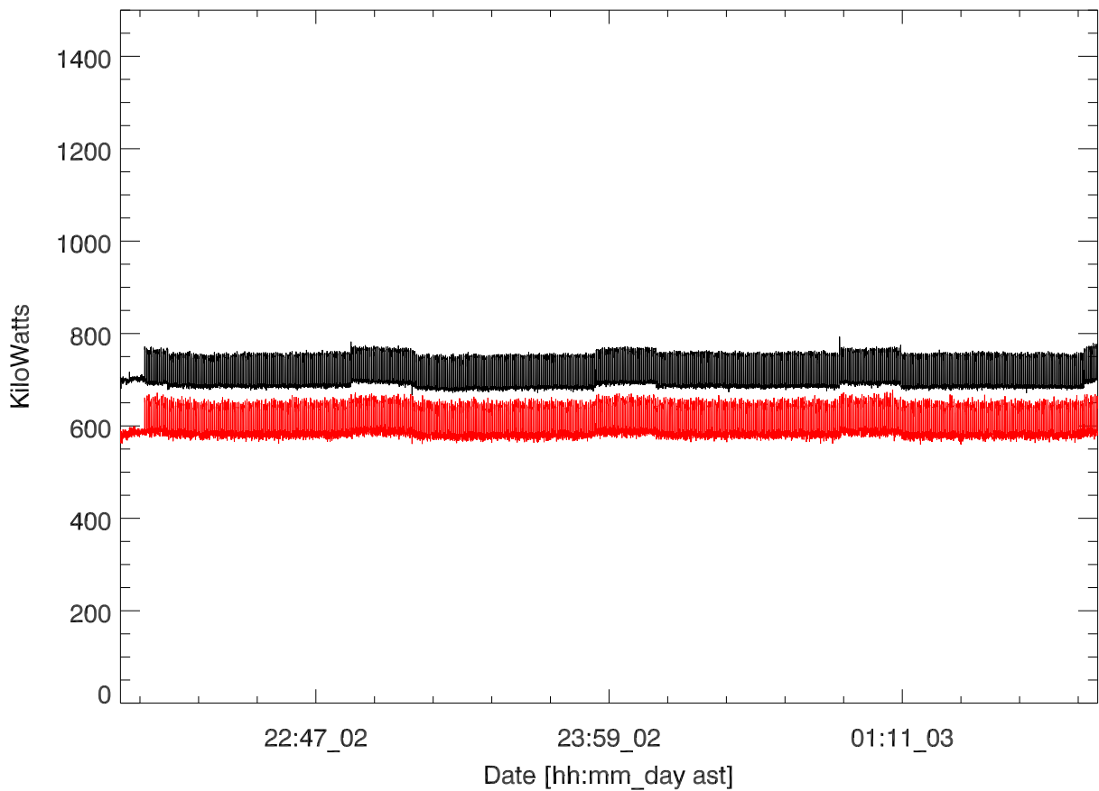
GD 430 Transmitted power for: 02oct16:T2689. Min-Chang Lee.
