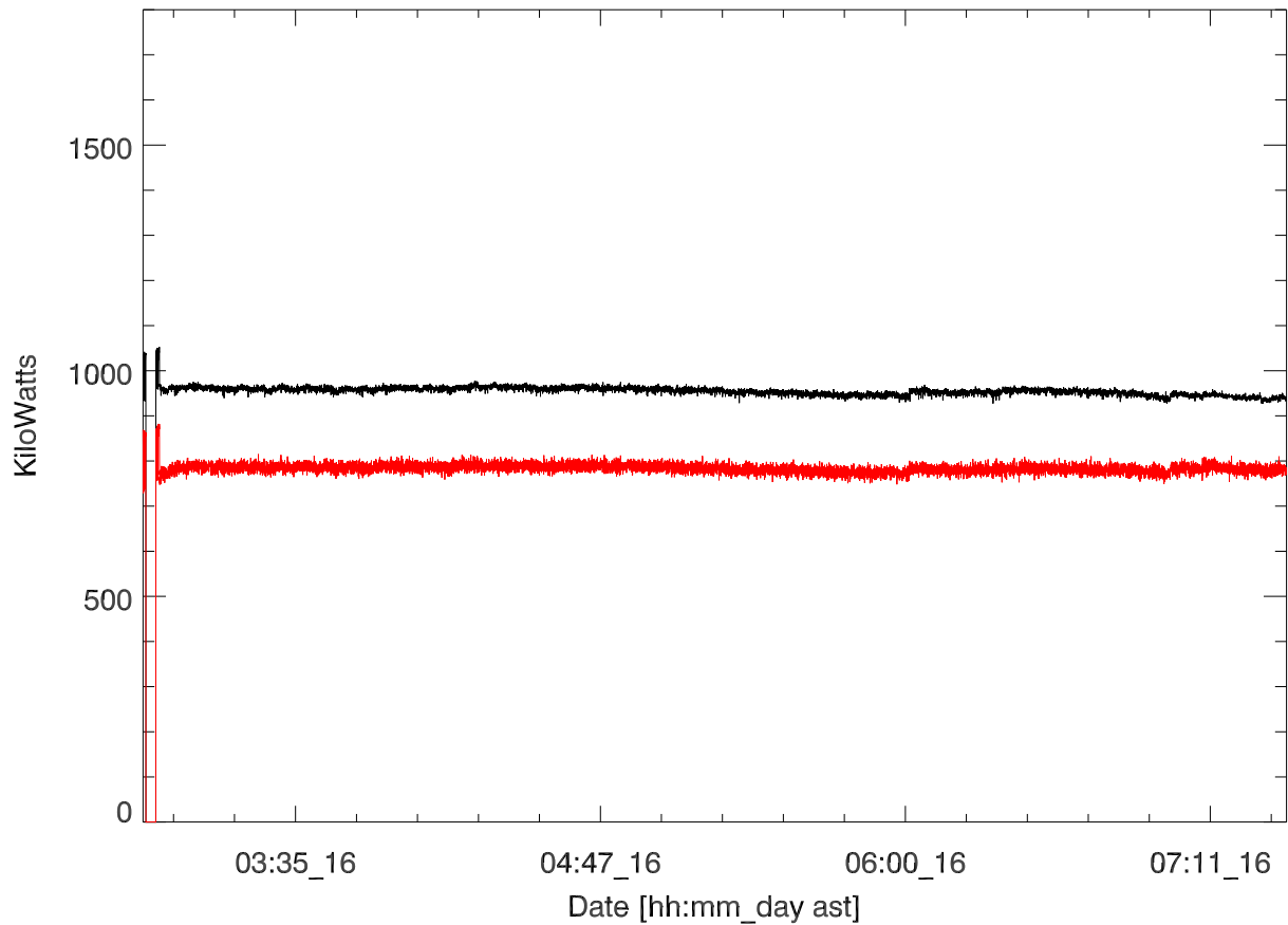
GD 430 Transmitted power for: 16mar17:T2869. Suman Ganguly
