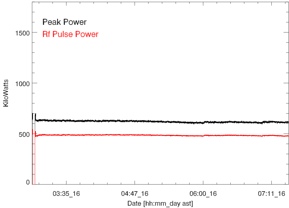
CH 430 Transmitted power for: 16mar17:T2869. Suman Ganguly
