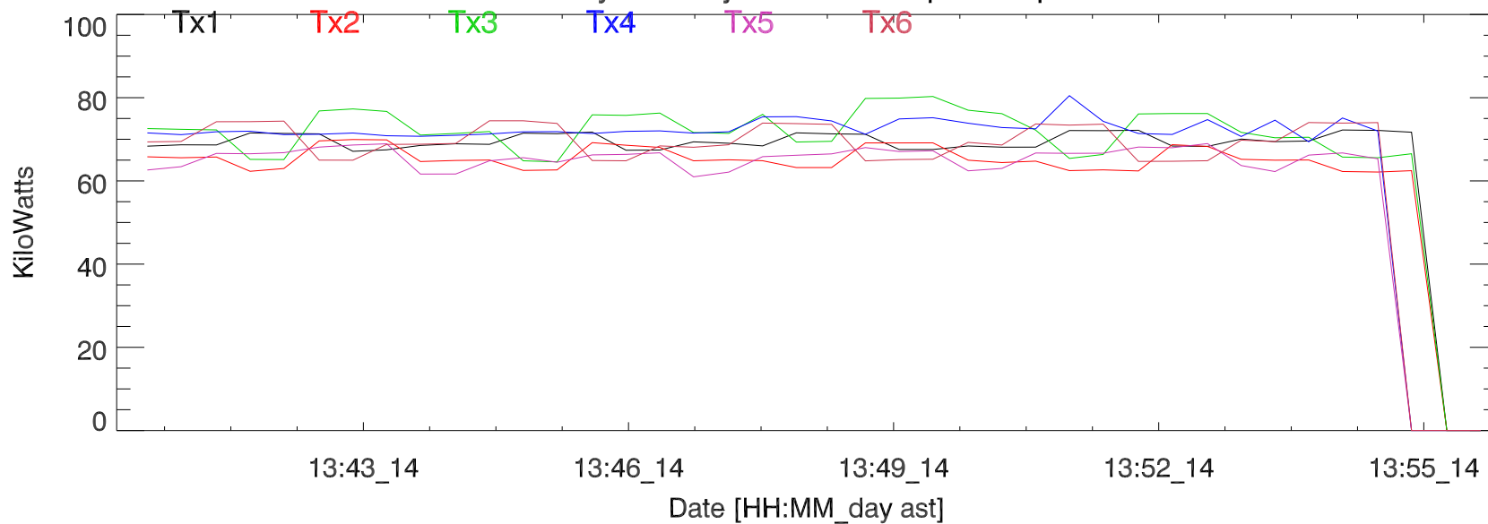
TxPwr by Tx. 14jun19:H3337 paul exp14.06
