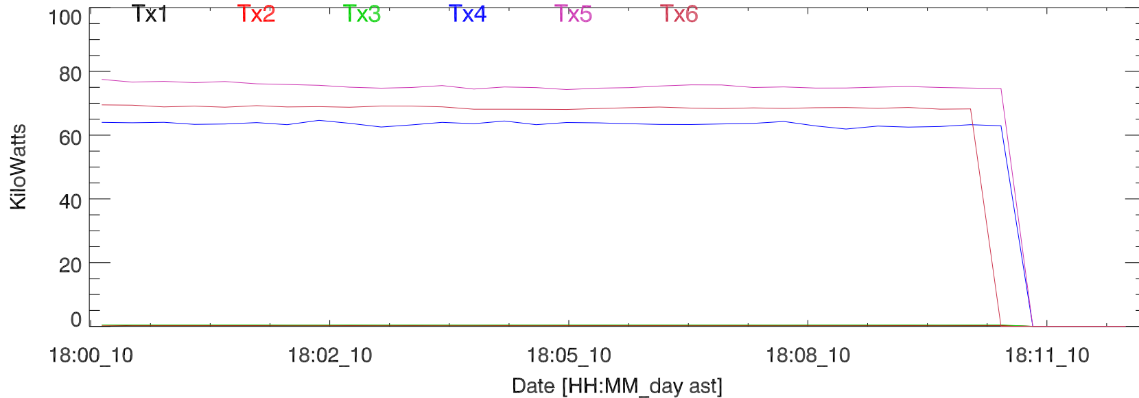
TxPwr by Tx. 10jun19:H3195 vladimir exp10.10
