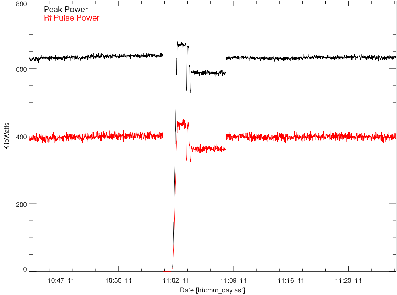
GD 430 Transmitted power for: 11jun19:H3337 paul exp11.03
