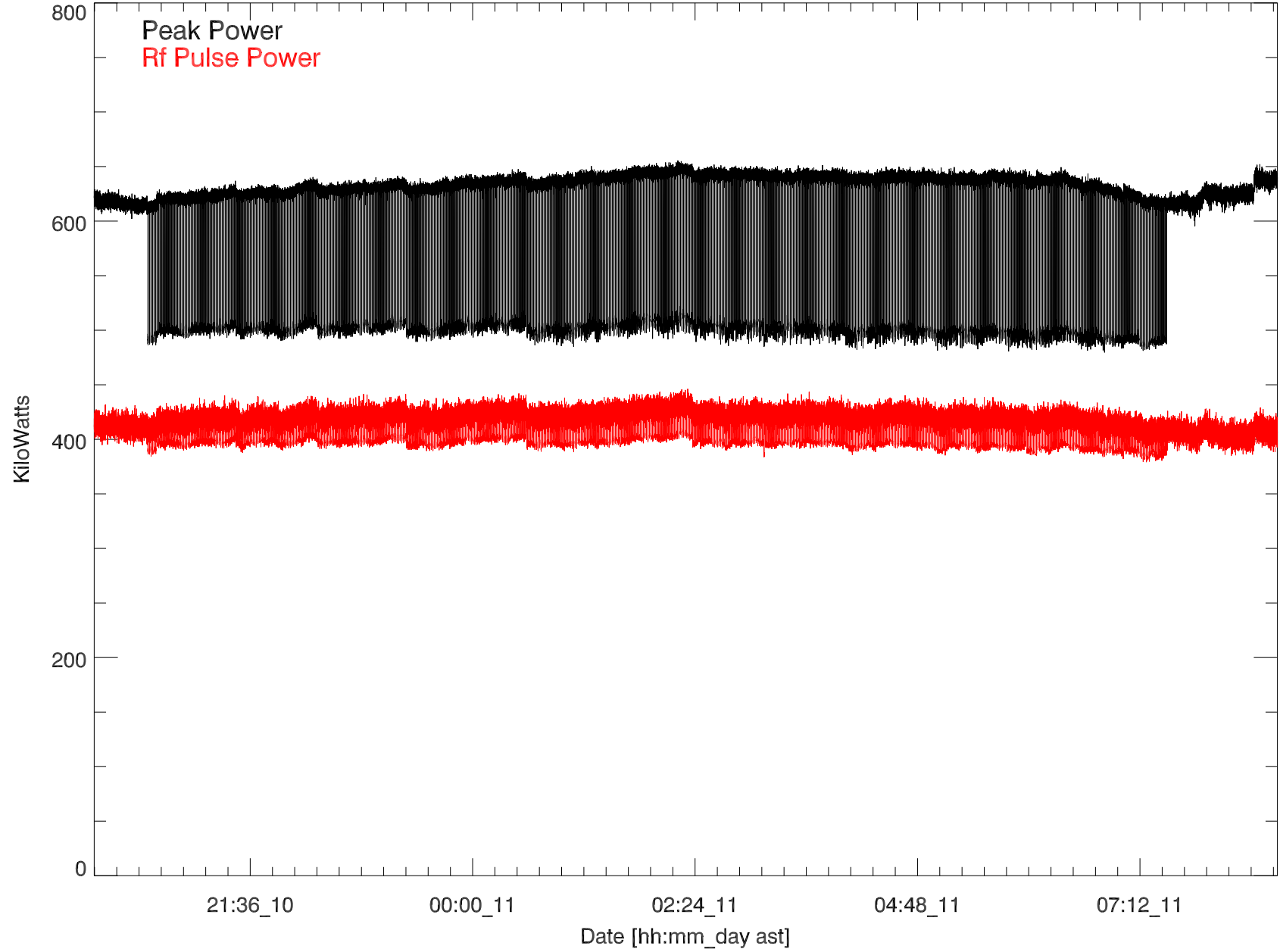
GD 430 Transmitted power for: 10jun19:T1193. suman (no hf) exp10.20
