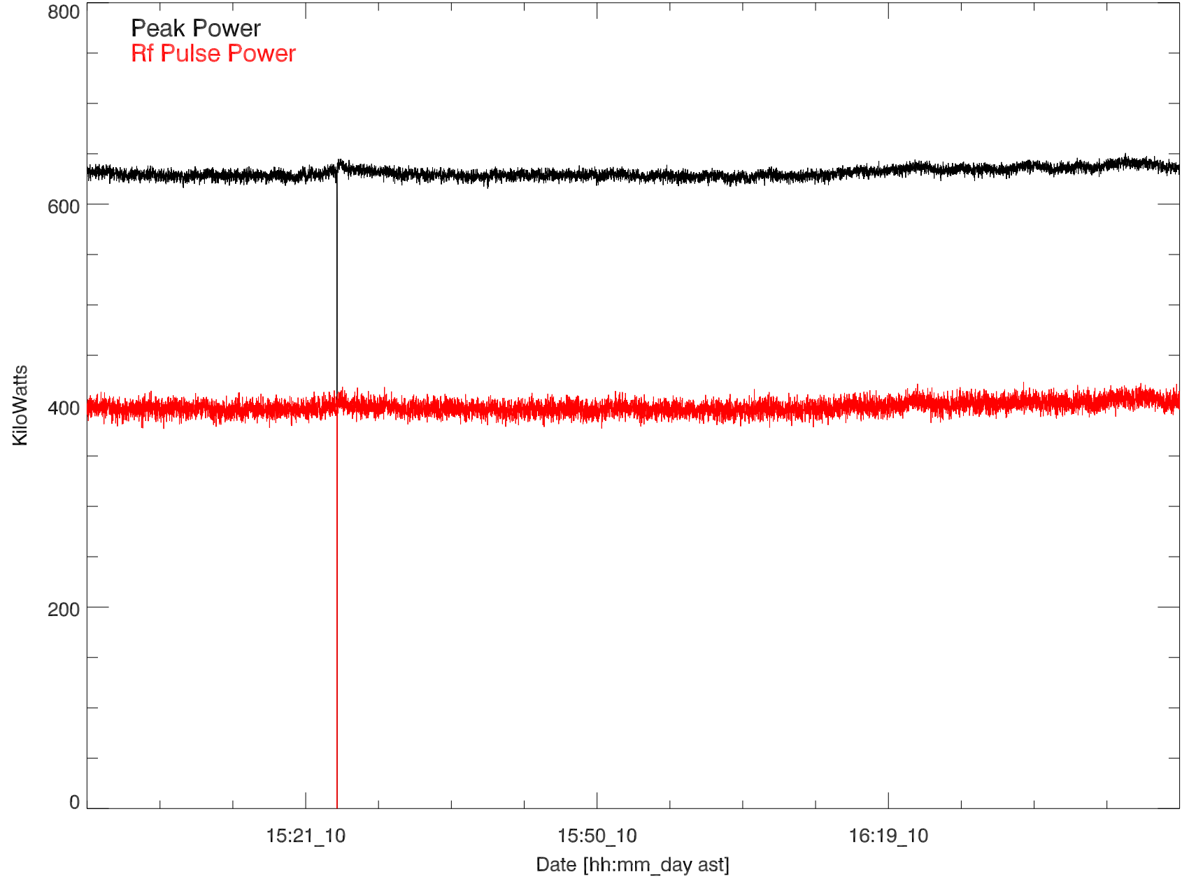
GD 430 Transmitted power for: 10jun19:H3195 vladimir exp10.07
