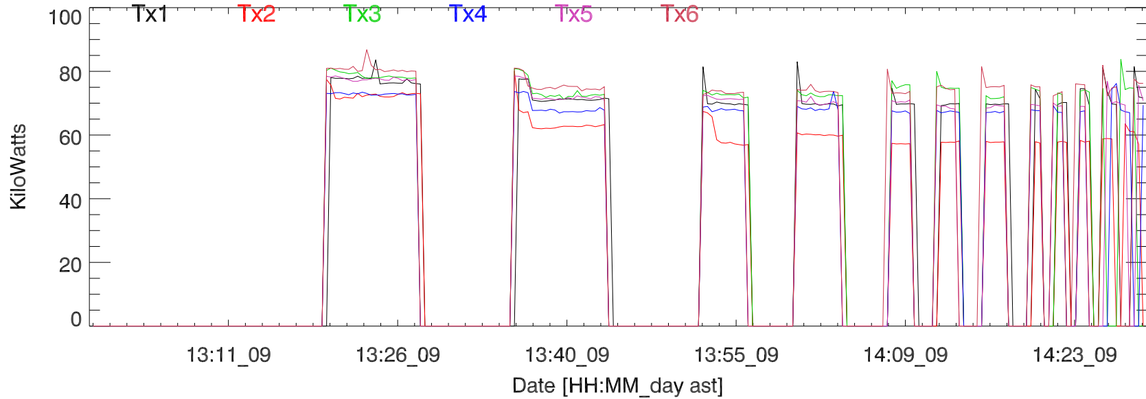
TxPwr by Tx. 09nov18:H3211
