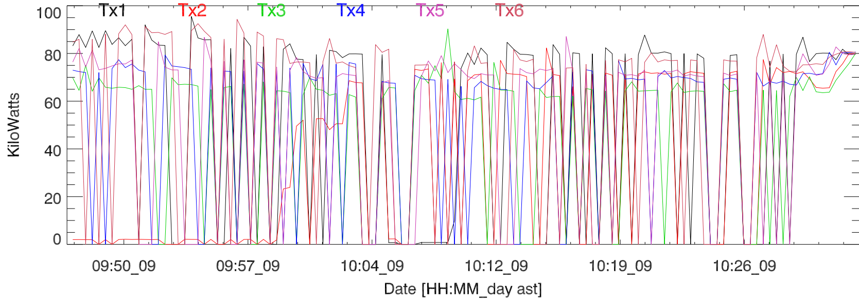
TxPwr by Tx. 09nov18:H3286
