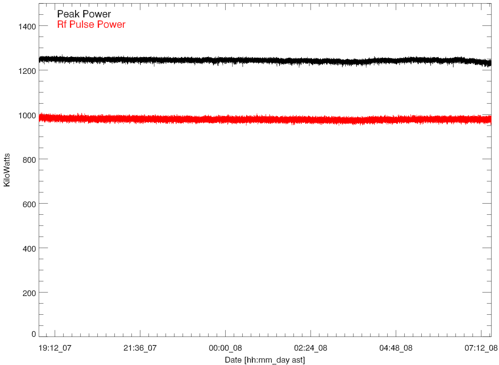
GD 430 Transmitted power for: 07nov18:T2374 (no hf)
