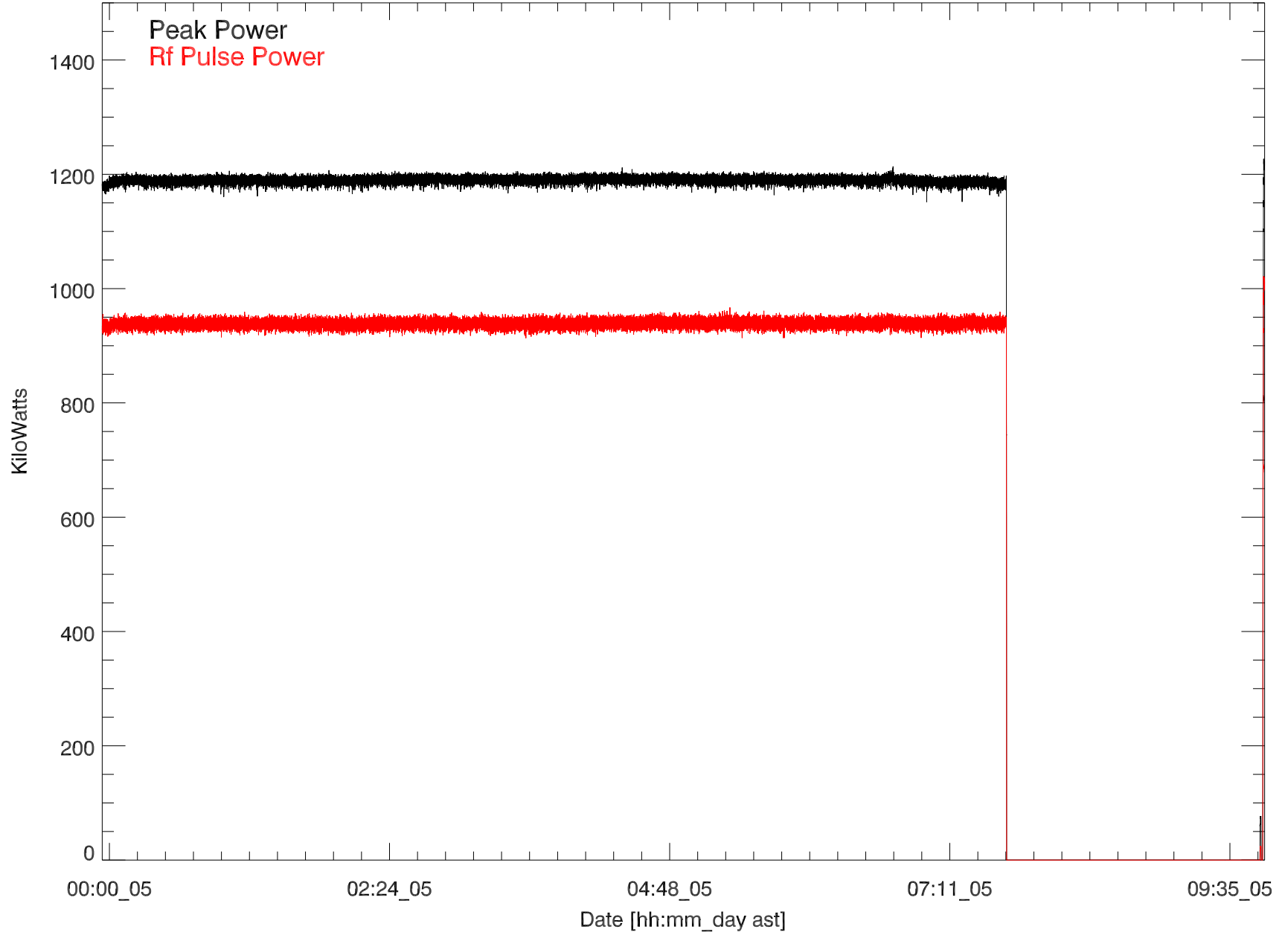
GD 430 Transmitted power for: 04nov18:T2374 (no hf)
