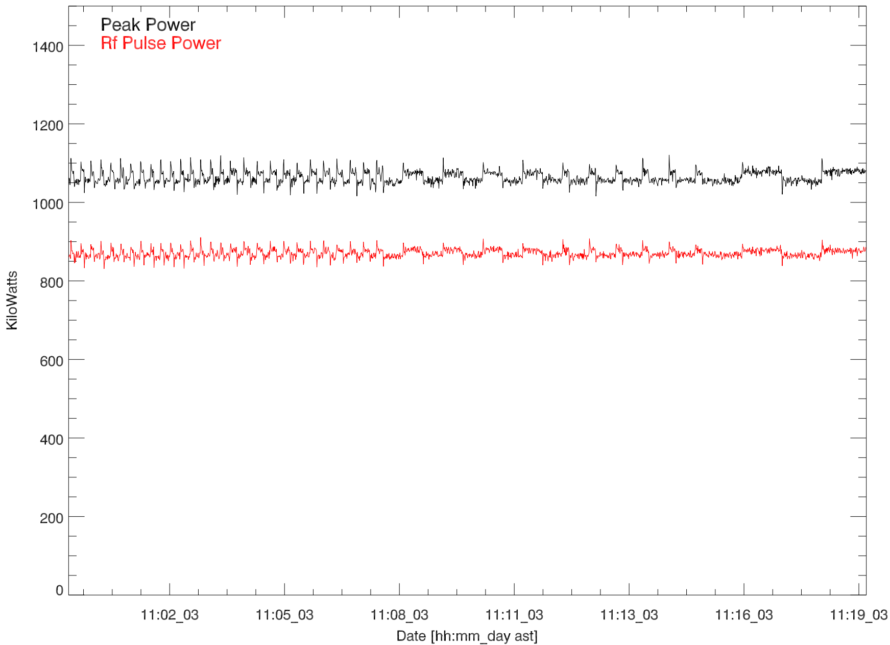
GD 430 Transmitted power for: 03nov18:H3286
