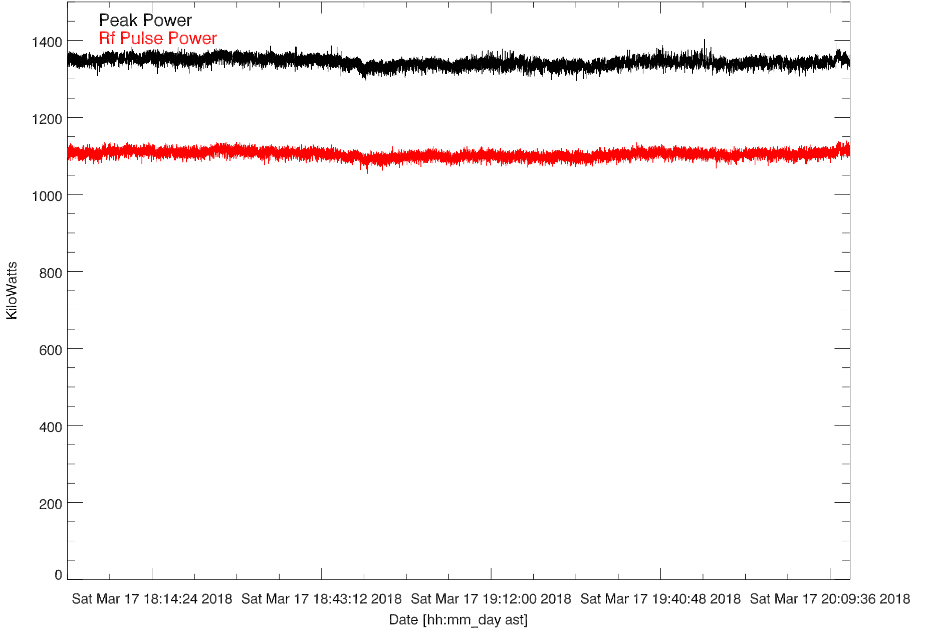
GD 430 Transmitted power for: 17mar18:H3249. Gennady
