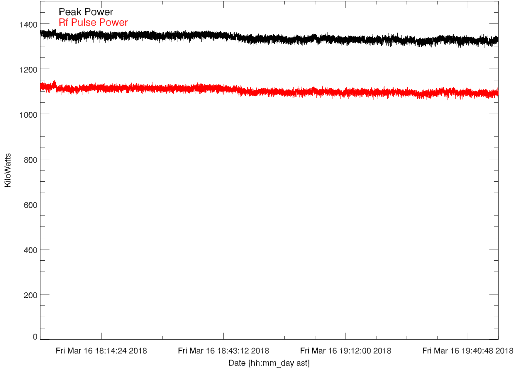
GD 430 Transmitted power for: 16mar18:H3249. Gennady
