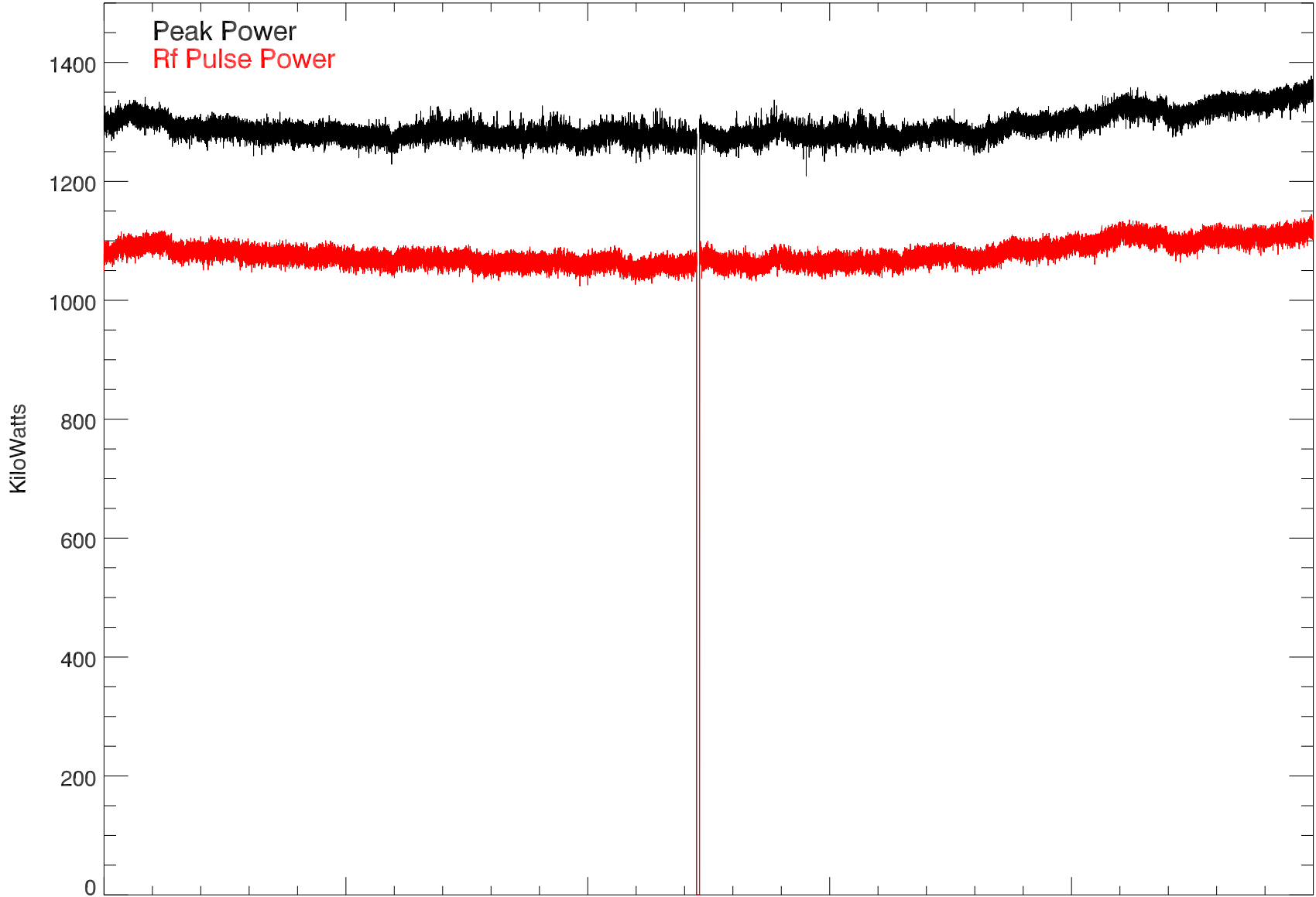
GD 430 Transmitted power for: 16mar18:H3252. Natasha
