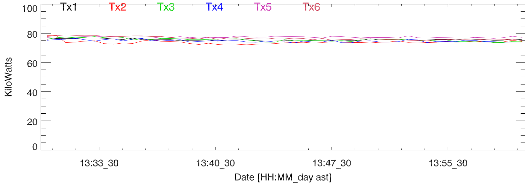
TxPwr by Tx. 30jul17: Paul
