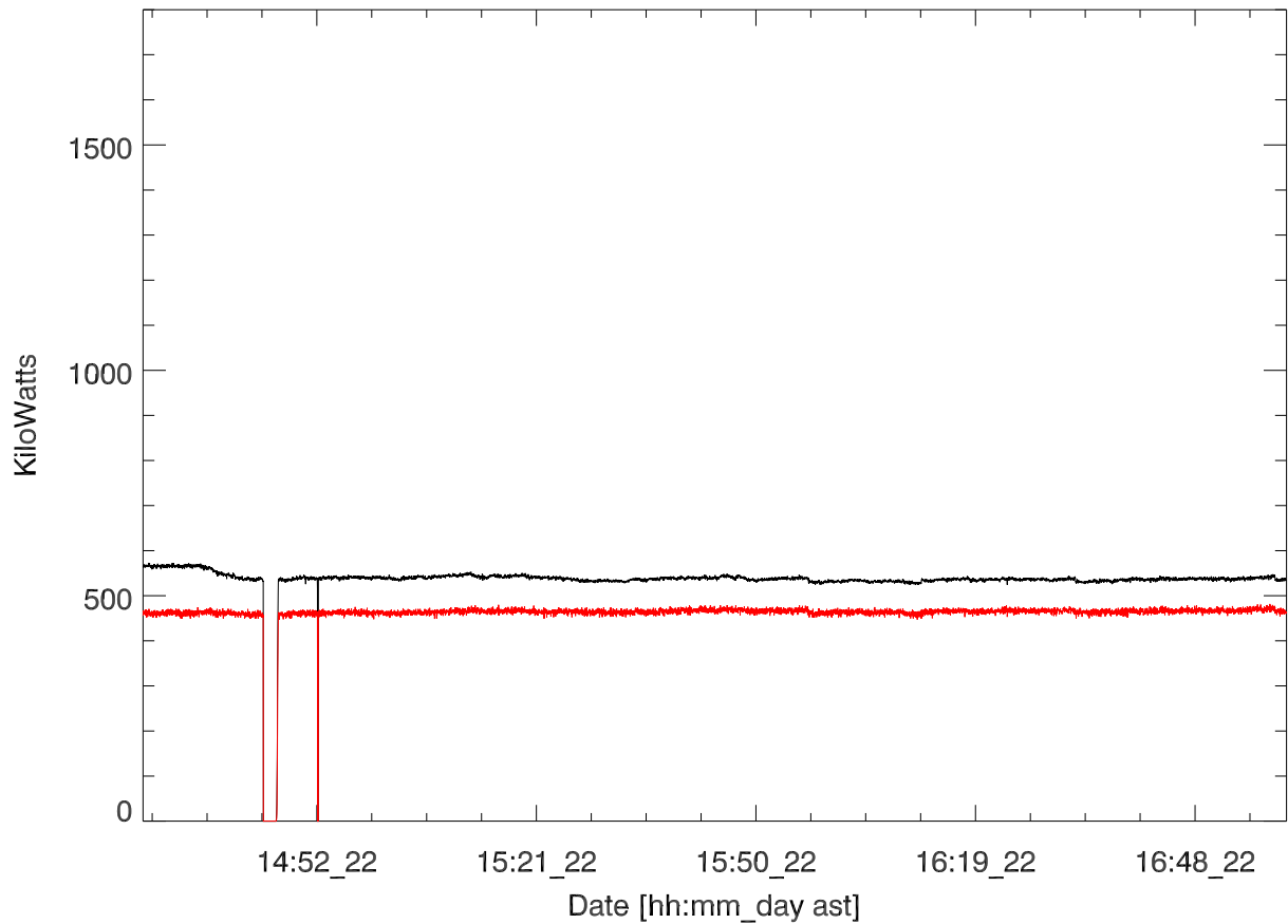
GD 430 Transmitted power for: 22may17:H3194. Natasha Jackson-Booth
