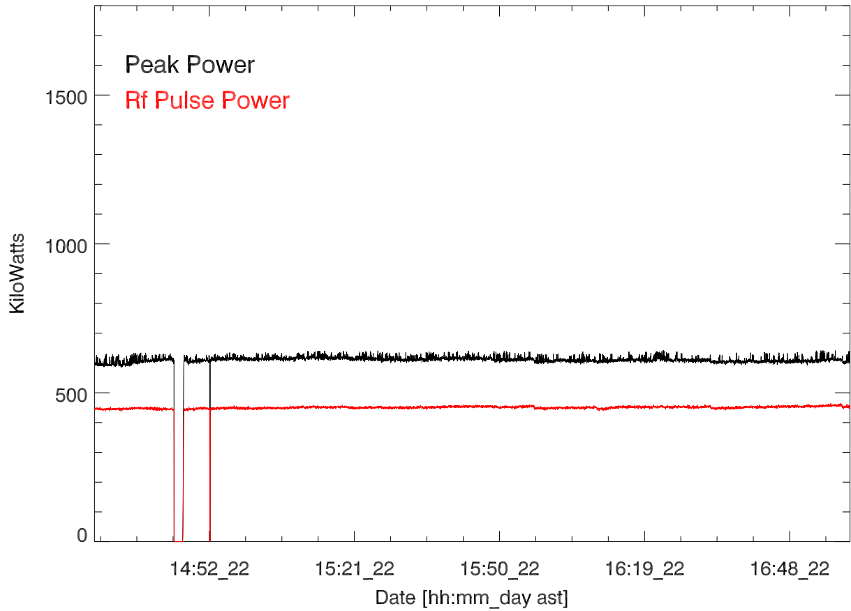
CH 430 Transmitted power for: 22may17:H3194. Natasha Jackson-Booth
