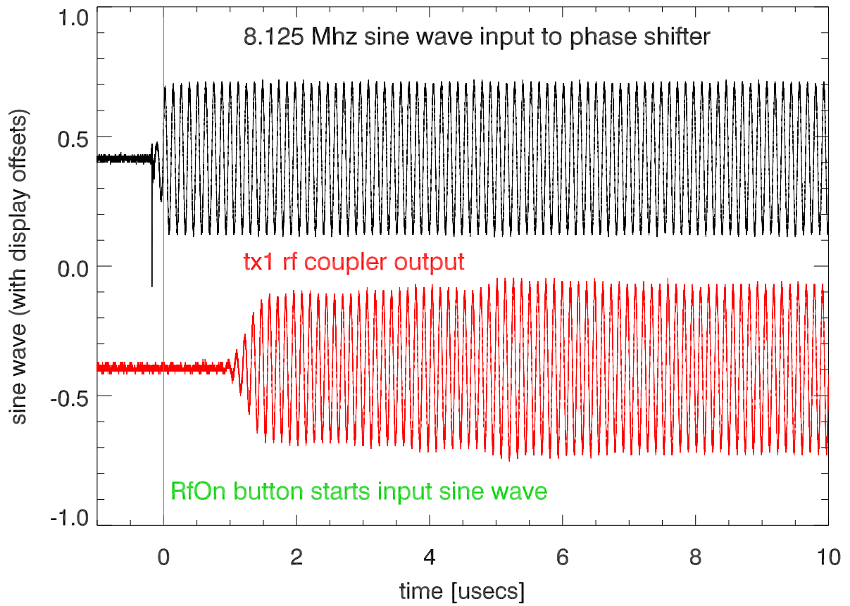
26aug18 srs sine wave driving hf and rf output
