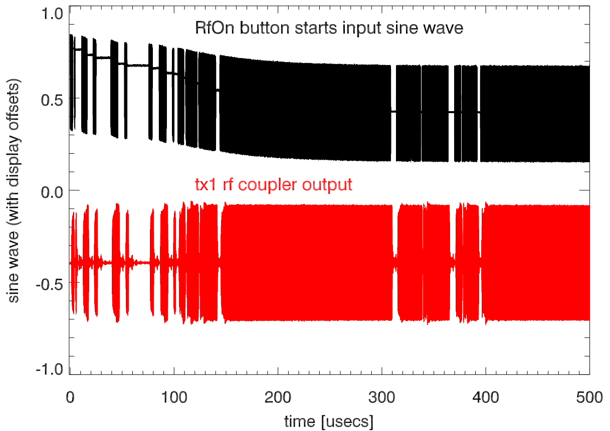
hp siggen sine wave driving hf and rf output
