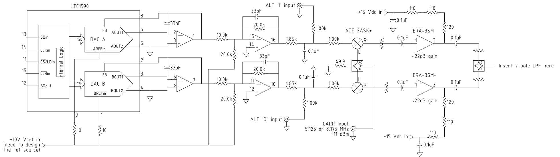
Analog Portion of hybrid phase adjuster for HF (1 channel of 6 shown)
