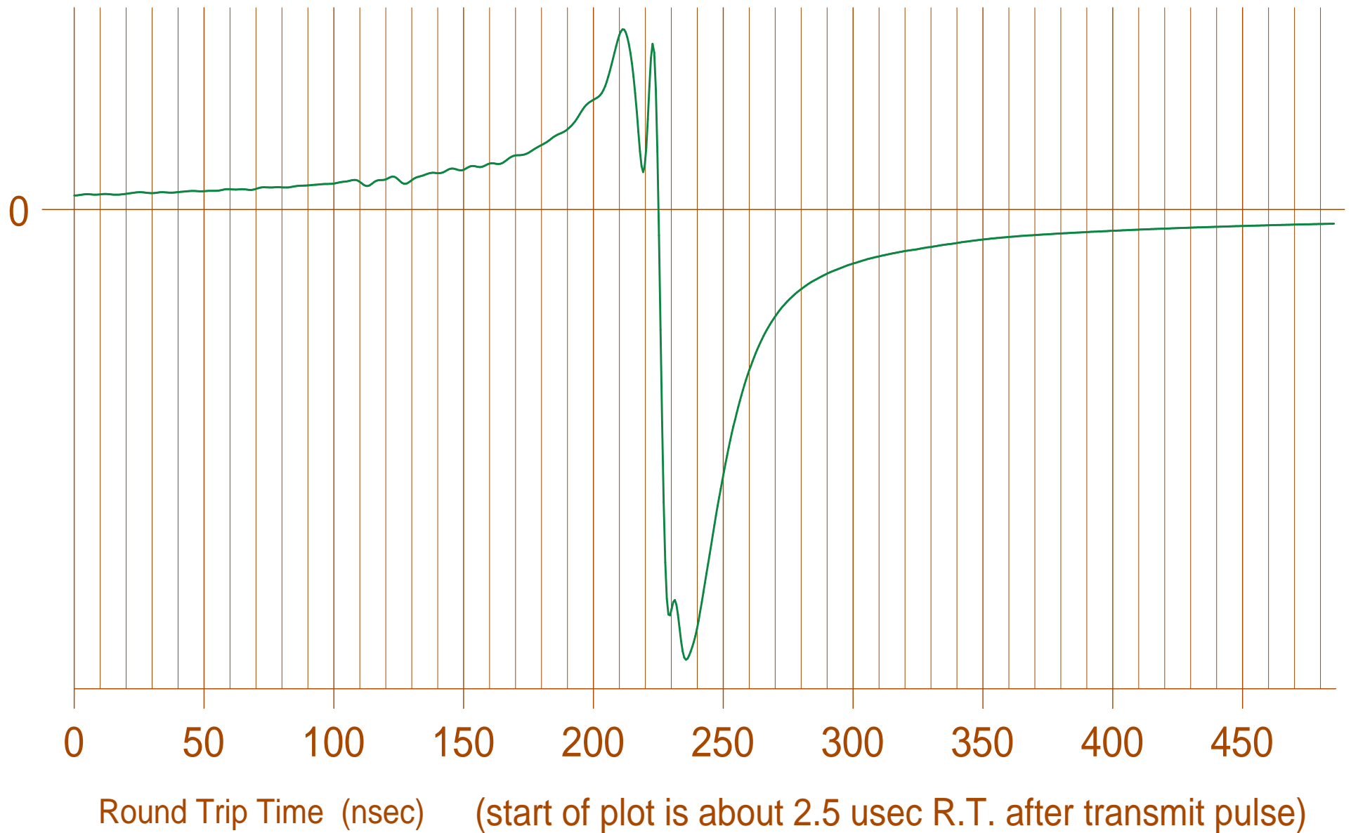
FD/TDR PLOT of FAR-END REFLECTION ON HF-3B (post-repair of arc damage incurred 3 June 2015; still something wrong)
