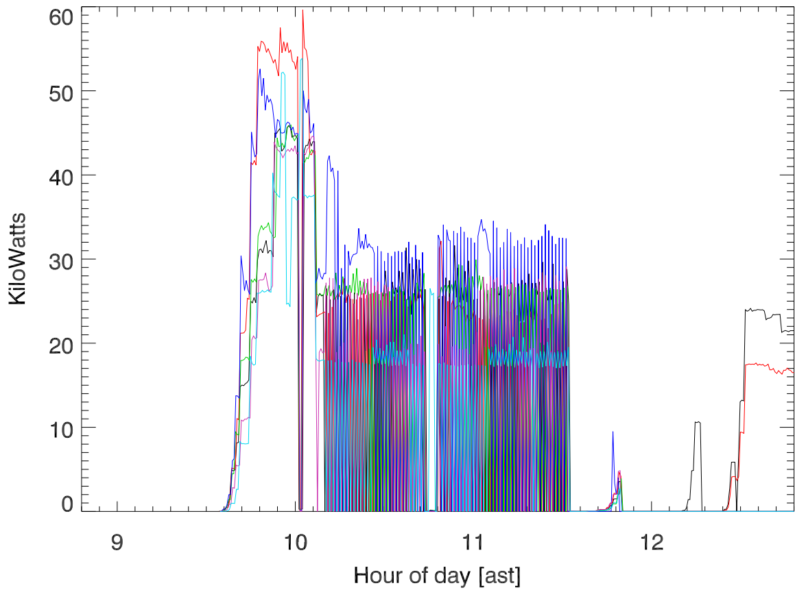
13sep16 Output power in KWatt by tx
