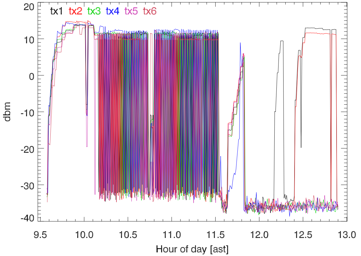
13sep16 8.175 Mhz tx power. rf coupler output
