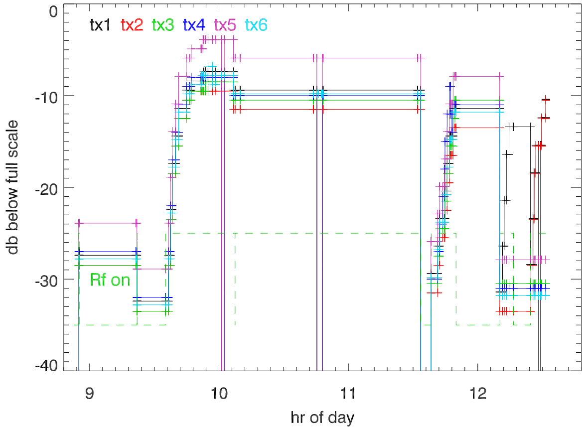
Entire run. synth drive amplitude
