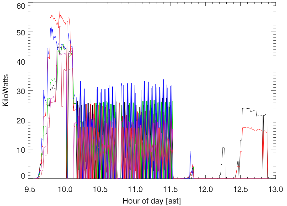
13sep16 Output power in KWatt by Tx
