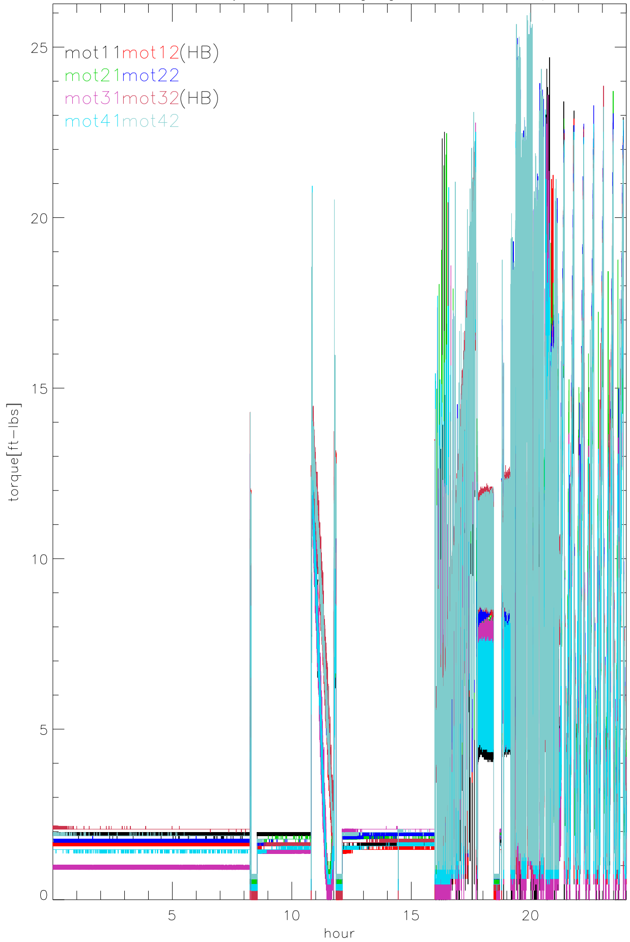
Dome summary for: 120523gregorian Motor Torques
