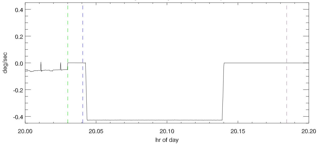
Az velocity from amplifier speed output
