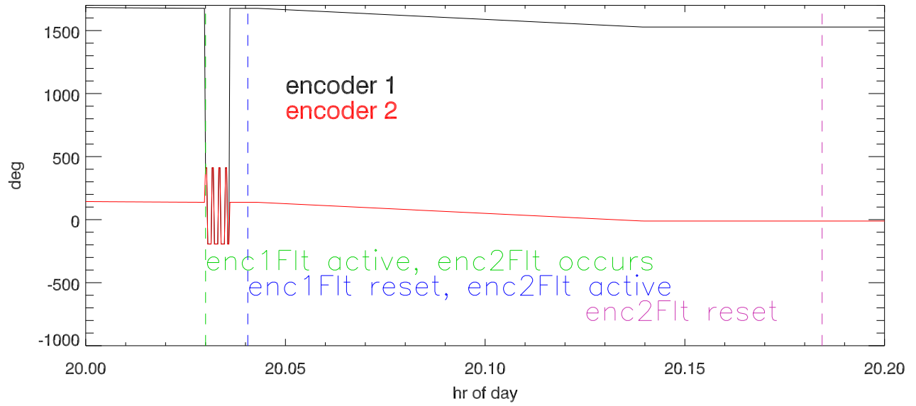
az encoder vs hour of day. blowup around 20:00
