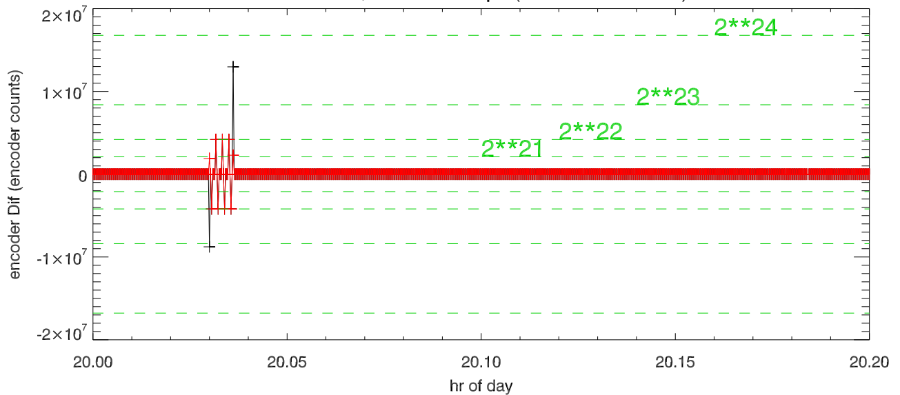
Encoder1, Encoder2 steps (in encoder counts)
